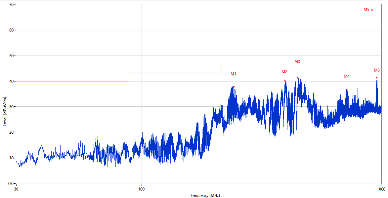
MIDDLE CHANNEL 30 MHz to 1 GHz, ANT H
