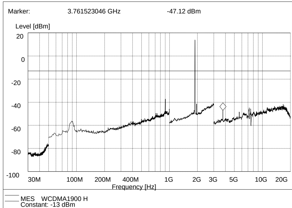
WCDMA 1900MHz, Test Antenna Horizontal
