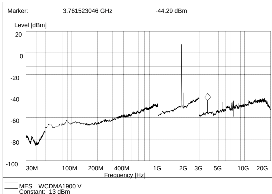
WCDMA 1900MHz, Test Antenna Vertical
