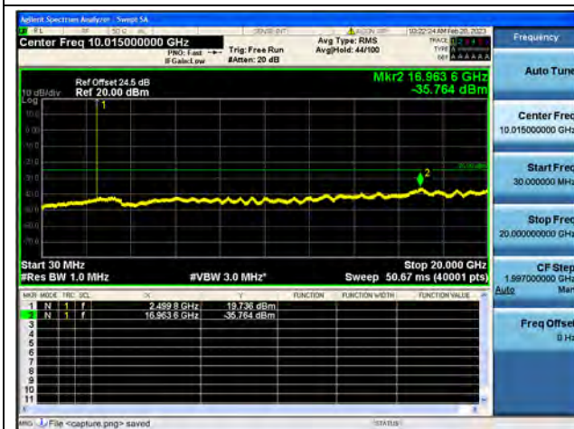
Band7-30M-20G / 5MHz / Low CH / 64QAM
