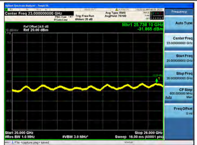
Band7-20G-26G / 5MHz / Low CH / 16QAM
