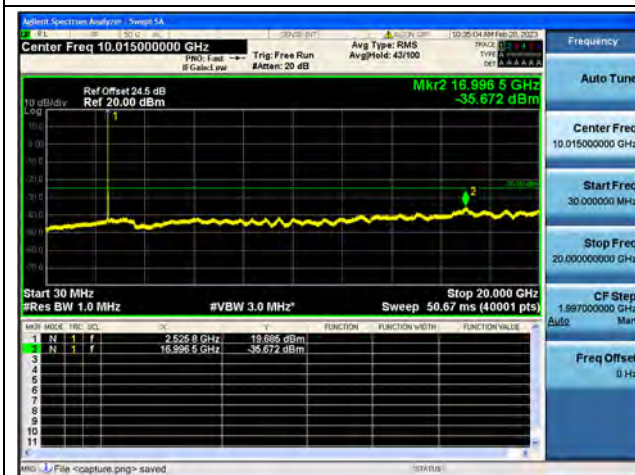
Band7-30M-20G / 20MHz / Mid CH / 64QAM
