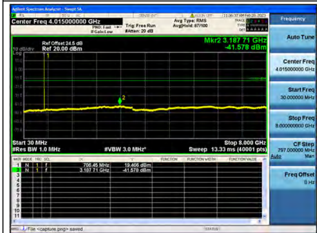
Band12 / 3MHz / Mid CH / 64QAM
