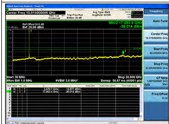
Band38-30M-20G / 20MHz / Low CH / 64QAM
