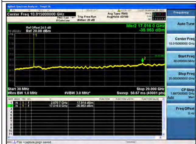
Band38-30M-20G / 20MHz / Low CH / 16QAM
