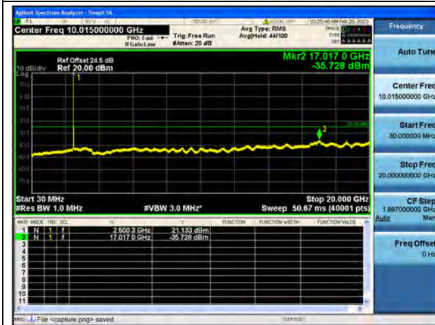
Band7-30M-20G / 10MHz / Low CH / 16QAM
