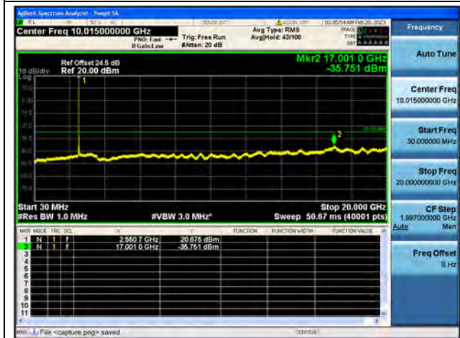
Band7-30M-20G / 20MHz / High CH / 16QAM
