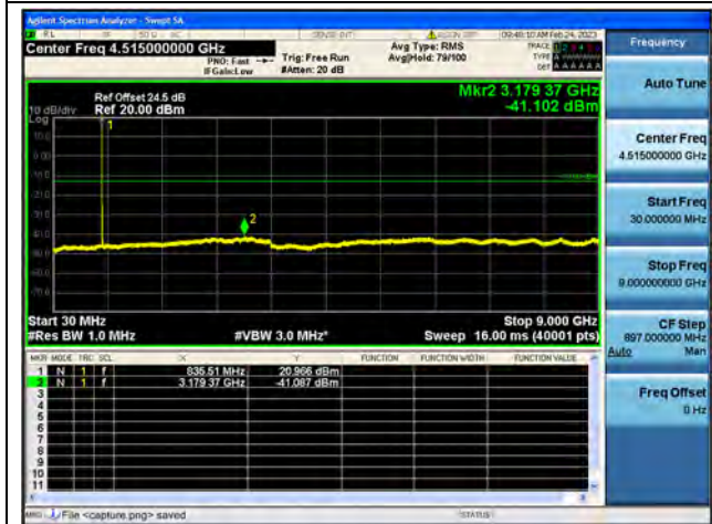
Band5 / 3MHz / Mid CH / 64QAM
