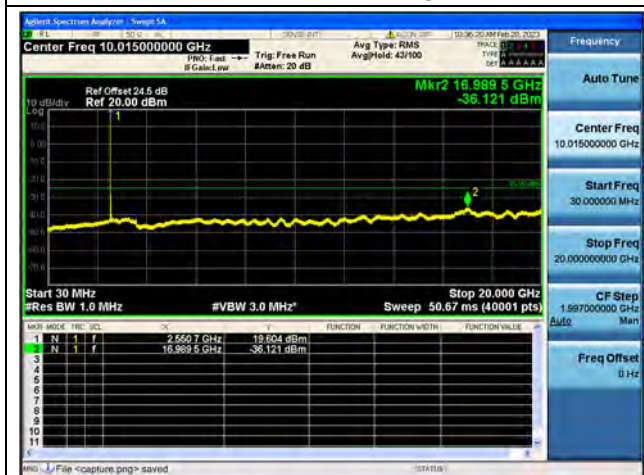
Band7-30M-20G / 20MHz / High CH / 64QAM
