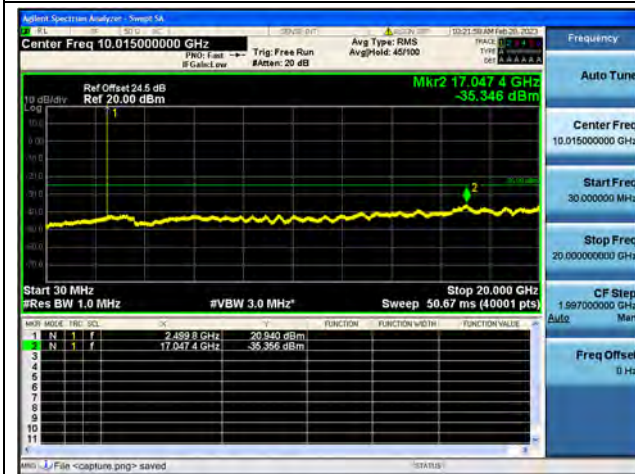
Band7-30M-20G / 5MHz / Low CH / 16QAM
