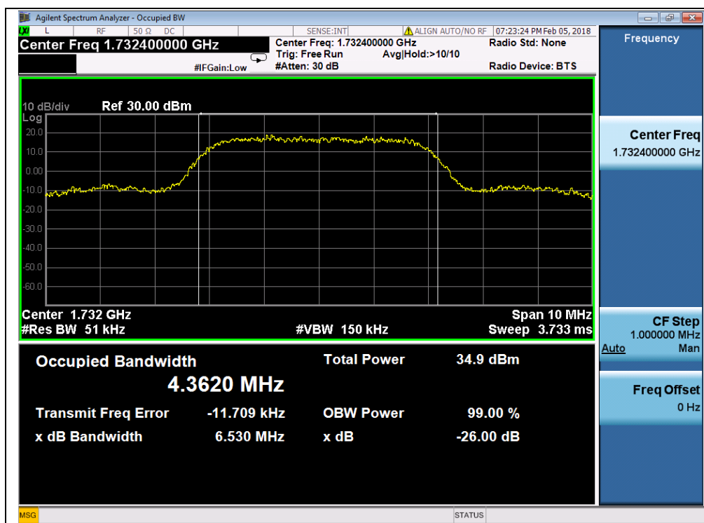
(Plot K2, HSDPA 1700 MHz, Channel = 1412)
