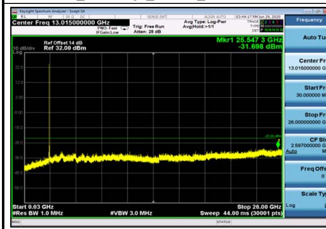
FDD07_MidRange_20MHz_30MHz~26GHz
