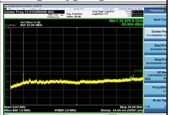
FDD07_MidRange_15MHz_30MHz~26GHz
