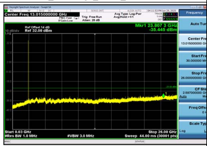
FDD07_MidRange_5MHz_30MHz~26GHz
