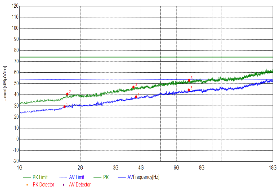
(Plot M: Test Antenna Horizontal 1G – 18G)
