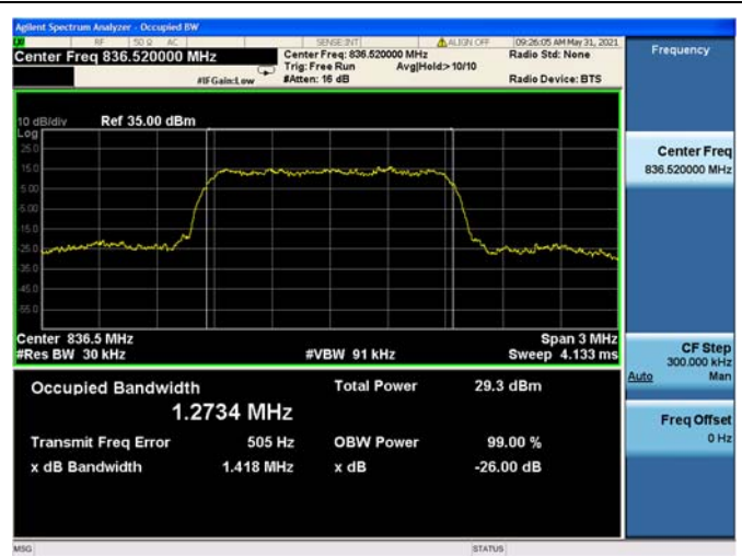
CDMA BC0 (1xRTT), CH384, 836.52MHz
