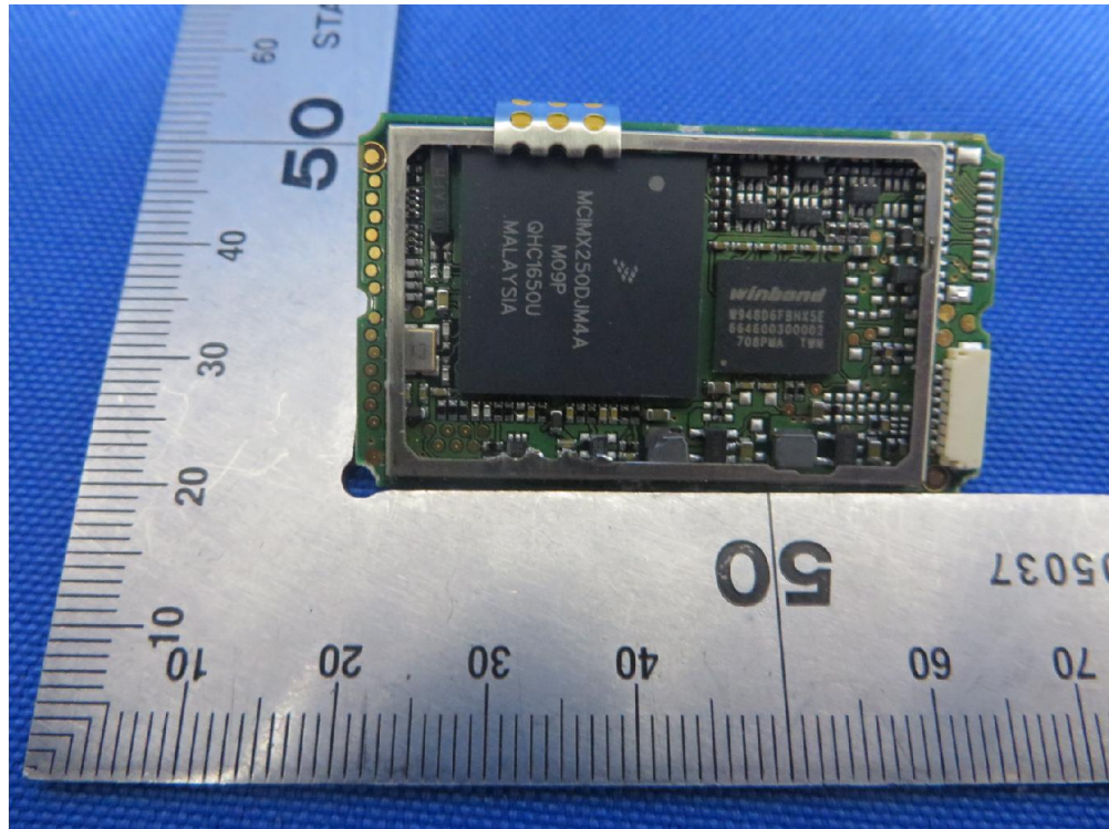
(27) EUT Photo
