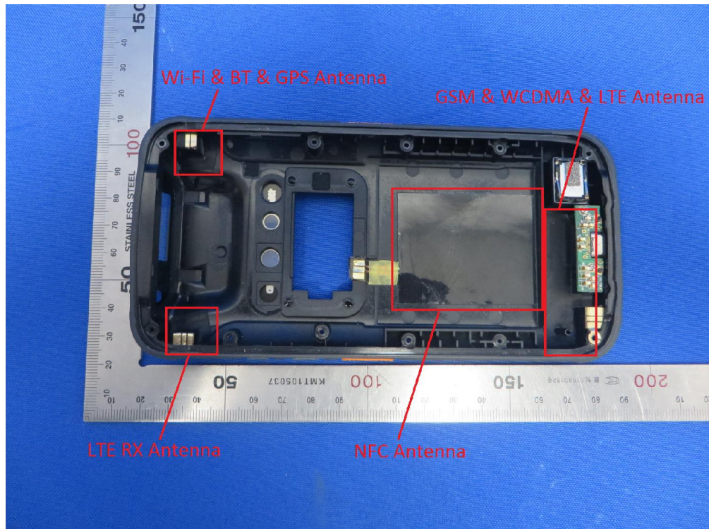
(23) EUT Photo
