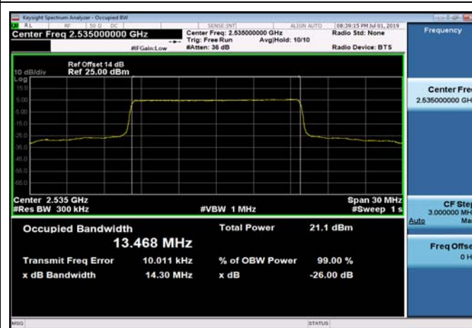
FDD07_MidRange_20MHz_2535MHz_QPSK
