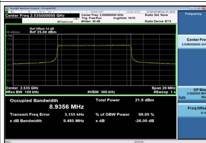
FDD07_MidRange_10_2535_QPSK
