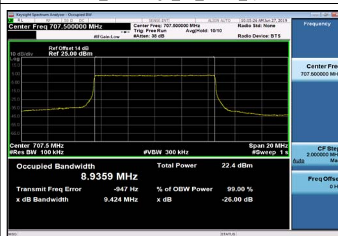
FDD12_MidRange_10_707.5_QPSK
