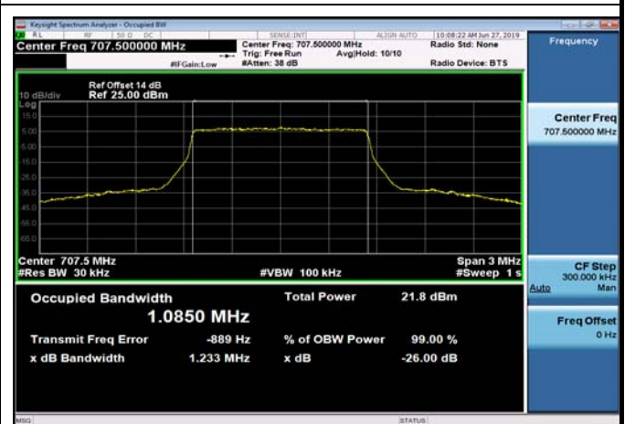
FDD12_MidRange_1.4_707.5_Q16
