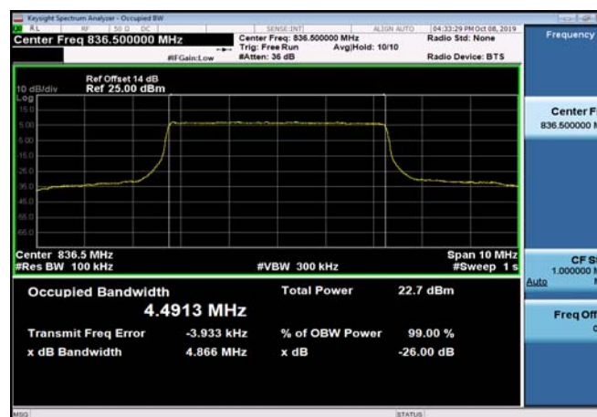
FDD05_MidRange_5MHz_836.5MHz_Q16
