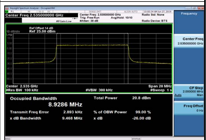
FDD07_MidRange_10_2535_Q16
