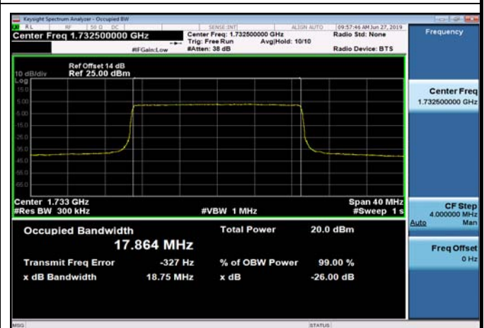
FDD04_MidRange_20_1732.5_Q16
