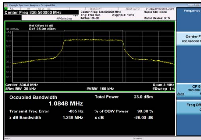
FDD05_MidRange_3MHz_836.5MHz_Q16
