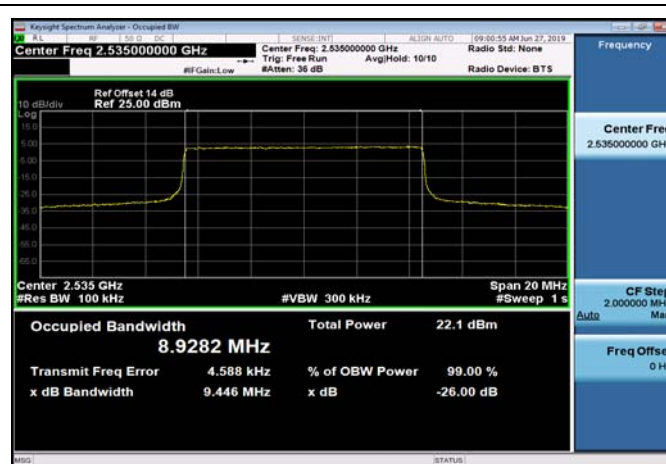
FDD07_MidRange_10MHz_2535MHz_QPSK
