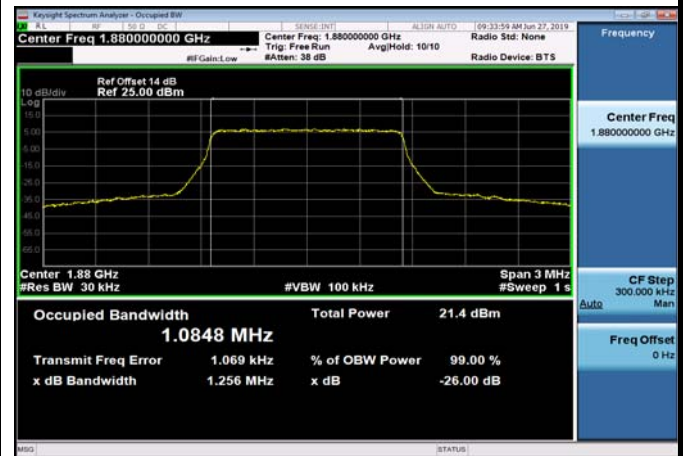
FDD02_MidRange_3_1880_Q16
