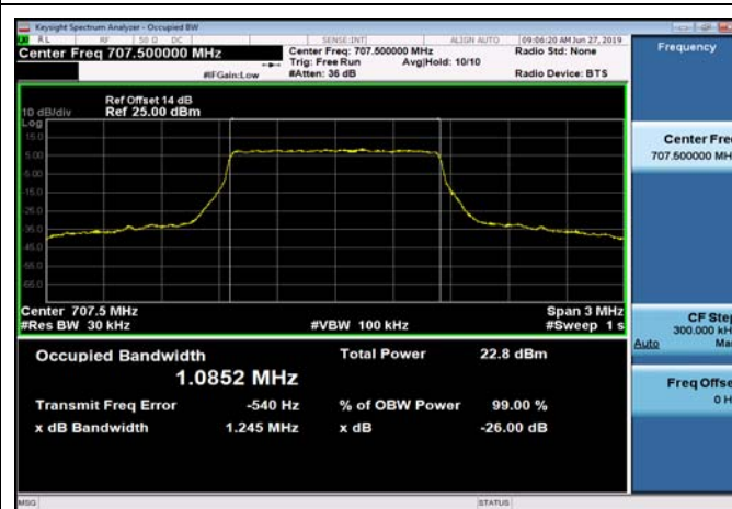
FDD12_MidRange_1.4MHz_707.5MHz_QPSK
