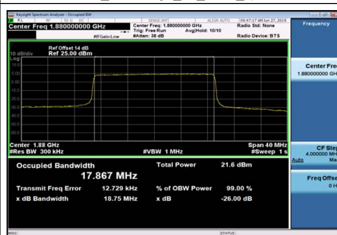
FDD02_MidRange_20_1880_QPSK
