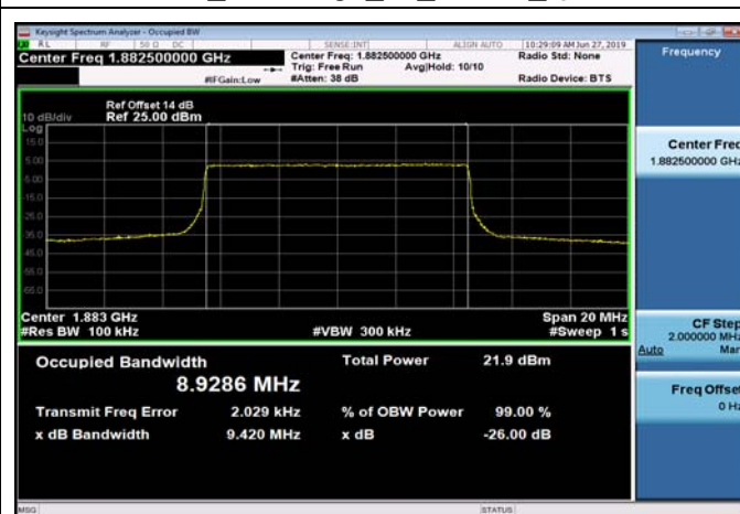
FDD25_MidRange_10_1882.5_QPSK
