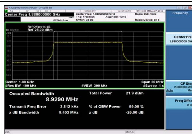
FDD02_MidRange_15_1880_QPSK
