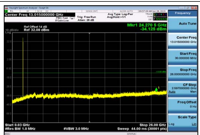
FDD25_LowRange_5MHz_30MHz~26GHz
