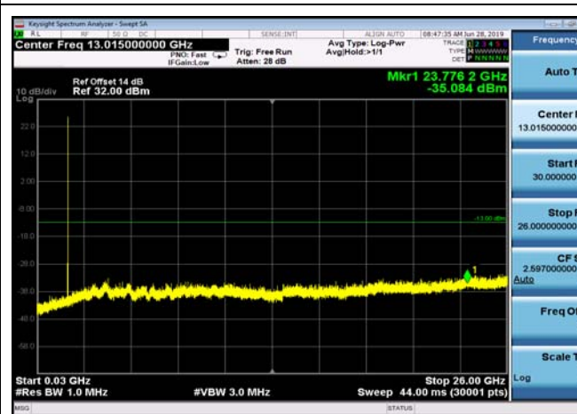
FDD04_MidRange_15MHz_30MHz~26GHz
