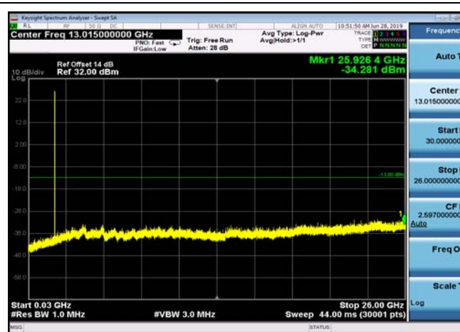
FDD25_LowRange_3MHz_30MHz~26GHz
