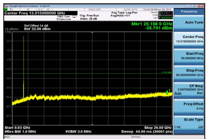
FDD02_HighRange_20MHz_30MHz~26GHz
