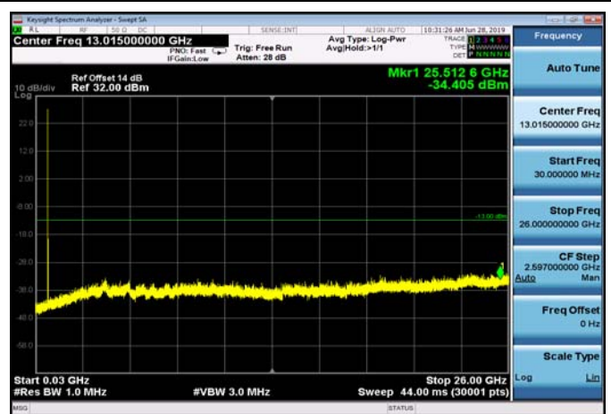
FDD12_MidRange_5MHz_30MHz~26GHz
