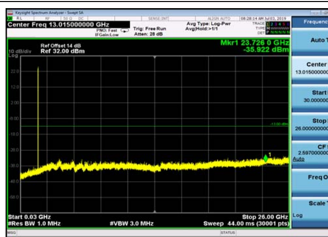
FDD66_HighRange_15MHz_30MHz~26GHz
