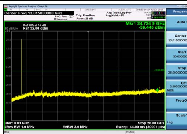
FDD66_HighRange_3MHz_30MHz~26GHz
