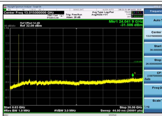
FDD66_LowRange_3MHz_30MHz~26GHz
