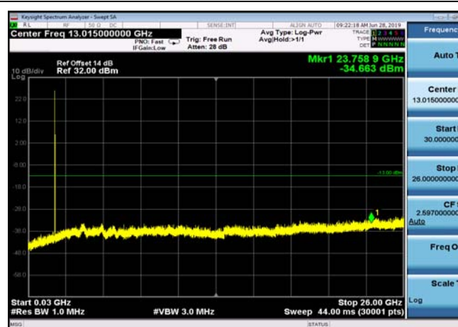
FDD02_MidRange_3MHz_30MHz~26GHz
