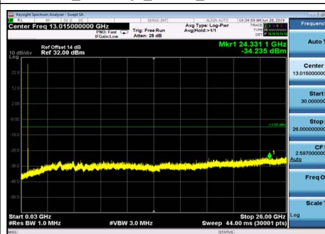
FDD17_MidRange_10MHz_30MHz~26GHz
