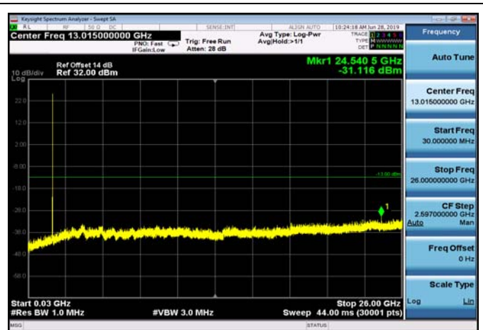
FDD04_MidRange_20MHz_30MHz~26GHz
