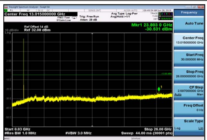
FDD02_HighRange_5MHz_30MHz~26GHz
