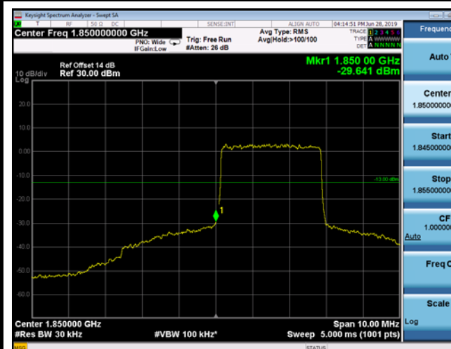
LowRange_FDD02_3MHz_1851.5_fullRB _Low_QPSK
