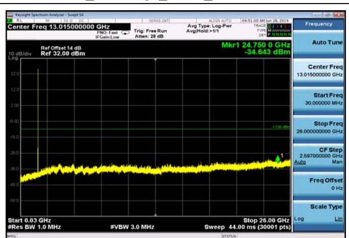
FDD04_MidRange_5MHz_30MHz~26GHz
