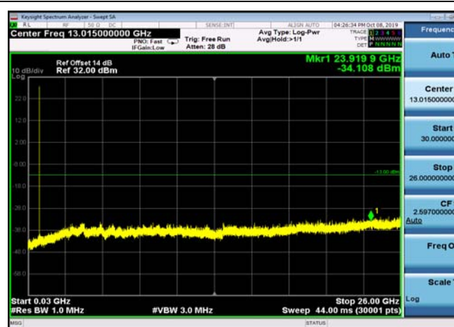
FDD05_LowRange_1.4MHz_30MHz~26GHz
