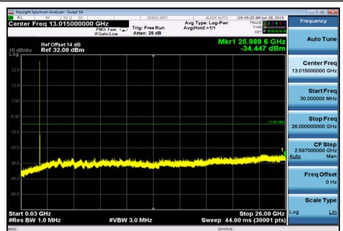
FDD02_MidRange_5MHz_30MHz~26GHz
