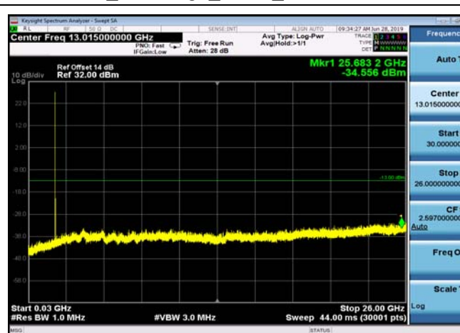
FDD25_MidRange_3MHz_30MHz~26GHz
