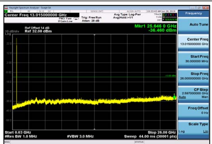
FDD12_HighRange_5MHz_30MHz~26GHz
