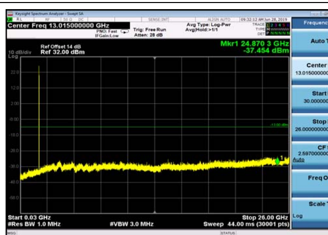
FDD25_LowRange_3MHz_30MHz~26GHz
