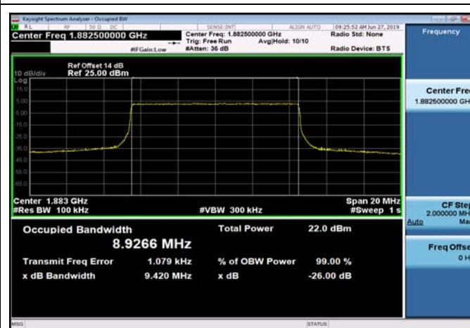
FDD25_MidRange_10MHz_1882.5MHz_QPSK
