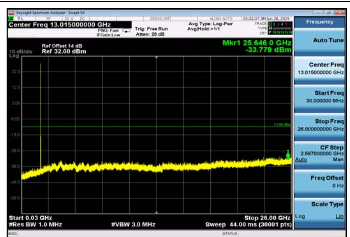
FDD02_MidRange_20MHz_30MHz~26GHz
