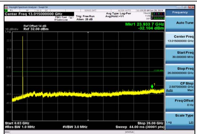
FDD25_LowRange_5MHz_30MHz~26GHz
