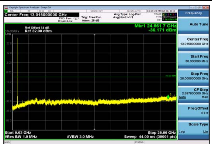
FDD05_LowRange_10MHz_30MHz~26GHz
