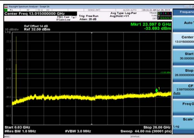
FDD12_LowRange_1.4MHz_30MHz~26GHz
