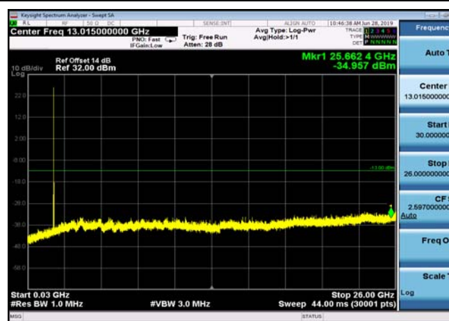
FDD02_MidRange_3MHz_30MHz~26GHz
