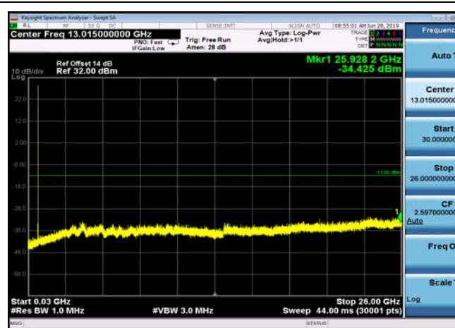
FDD12_HighRange_3MHz_30MHz~26GHz
