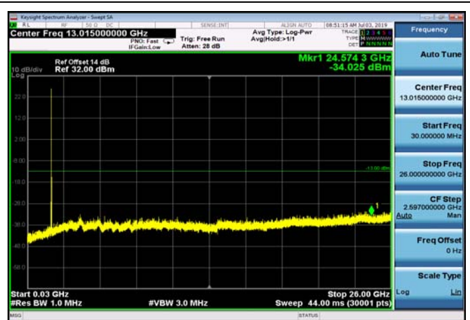
FDD66_MidRange_3MHz_30MHz~26GHz
