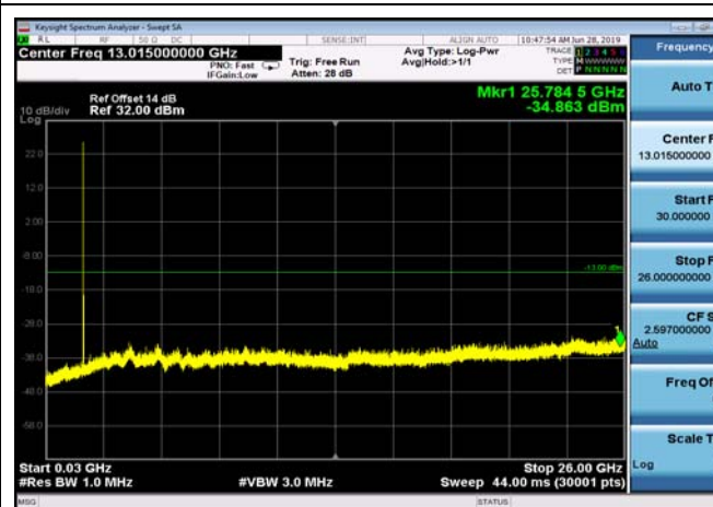
FDD04_LowRange_3MHz_30MHz~26GHz
