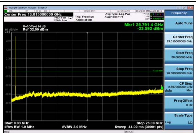
FDD12_LowRange_10MHz_30MHz~26GHz
