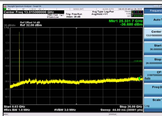
FDD02_MidRange_15MHz_30MHz~26GHz
