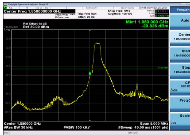
LowRange_FDD02_3MHz_1851.5_fullRB _Low_QPSK
