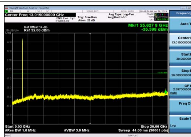
FDD04_MidRange_3MHz_30MHz~26GHz
