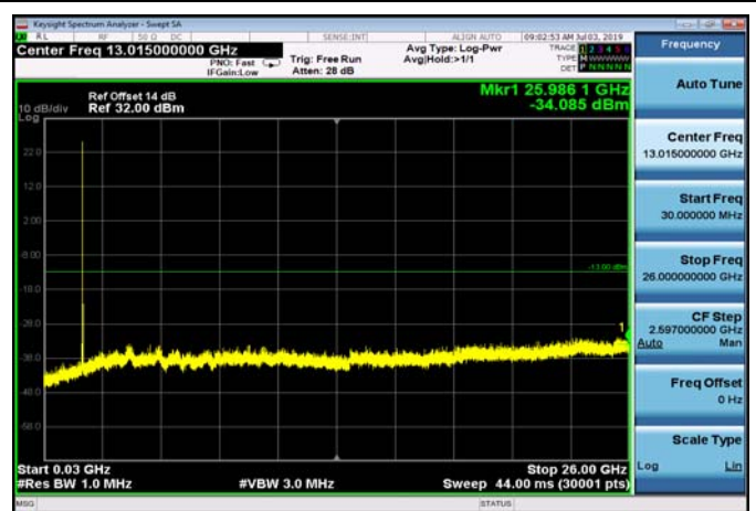
FDD66_HighRange_5MHz_30MHz~26GHz
