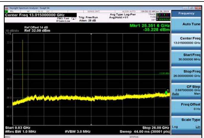
FDD04_LowRange_5MHz_30MHz~26GHz
