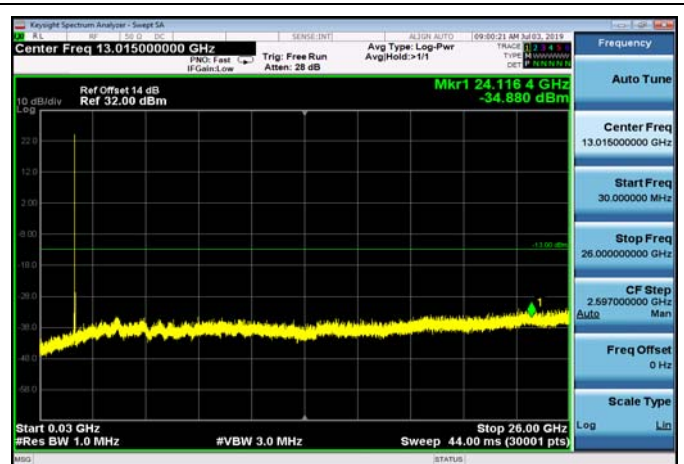
FDD66_MidRange_5MHz_30MHz~26GHz
