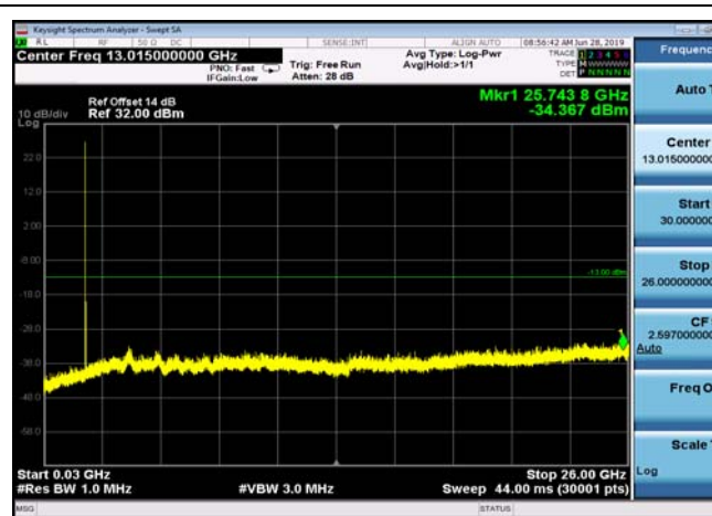
FDD25_MidRange_15MHz_30MHz~26GHz
