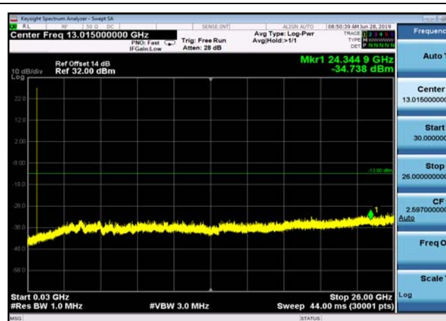
FDD12_LowRange_1.4MHz_30MHz~26GHz
