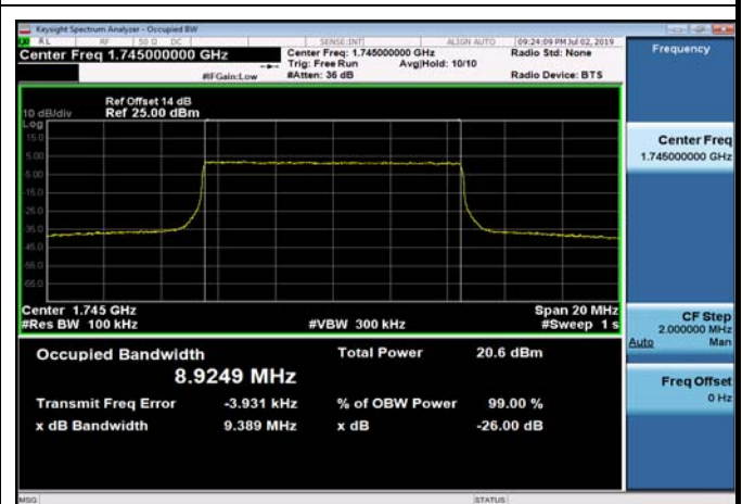
FDD66_MidRange_10MHz_1745MHz_Q16
