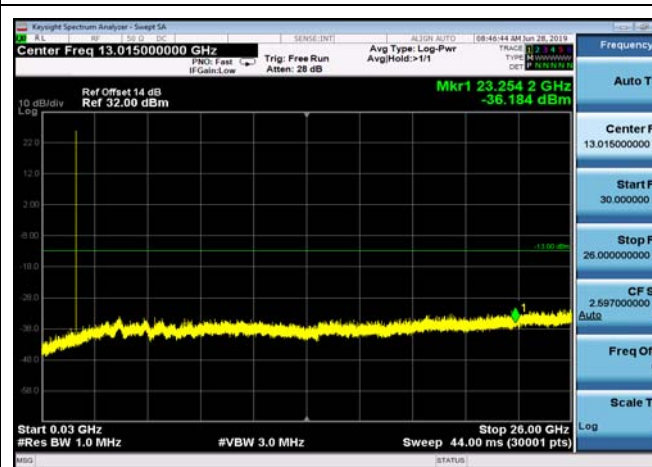
FDD04_LowRange_15MHz_30MHz~26GHz
