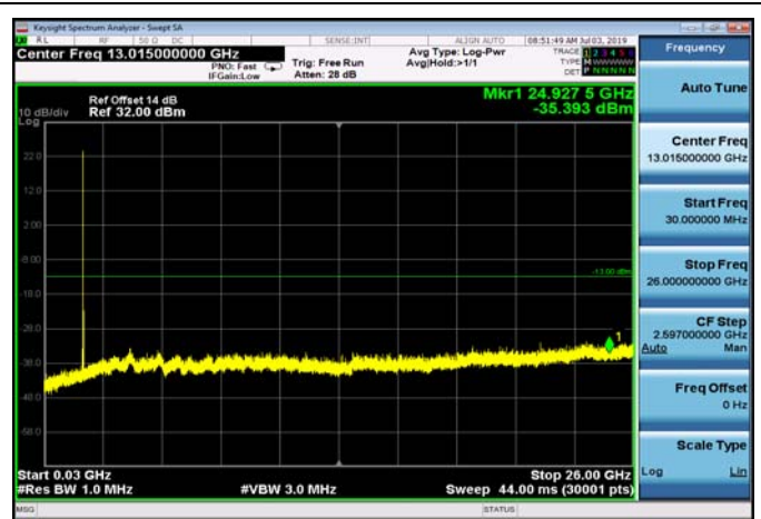
FDD66_HighRange_20MHz_30MHz~26GHz
