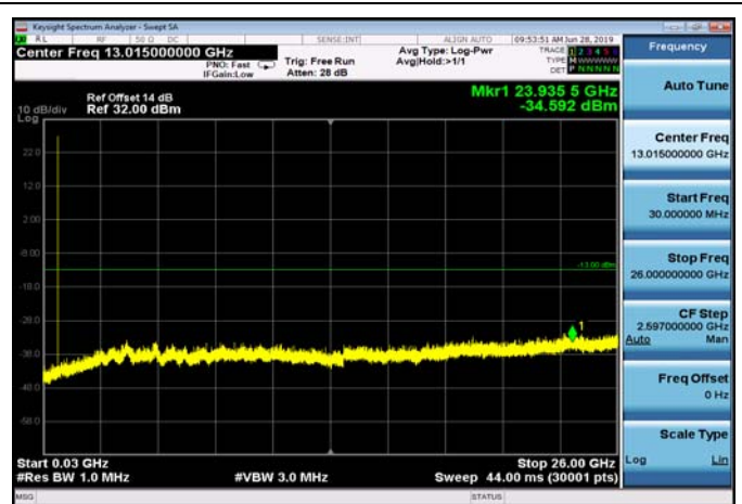
FDD12_MidRange_10MHz_30MHz~26GHz
