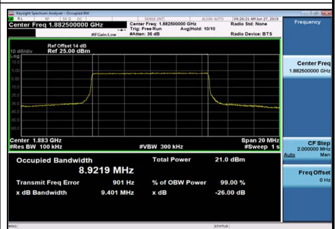
FDD25_MidRange_10MHz_1882.5MHz_Q16
