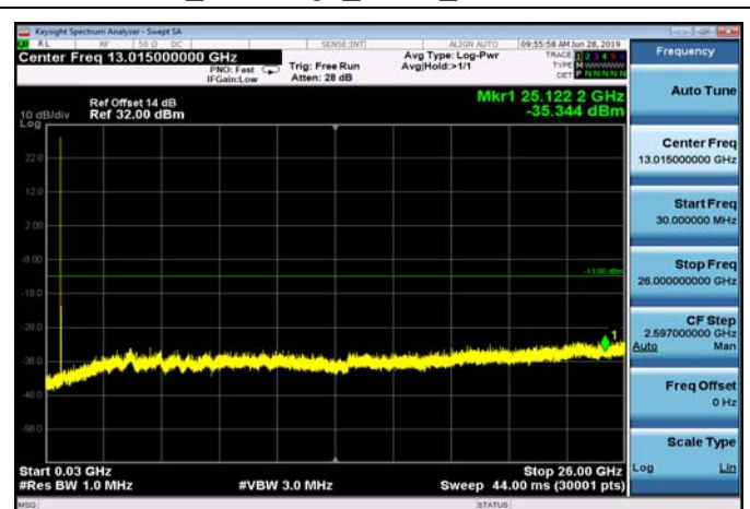
FDD17_MidRange_5MHz_30MHz~26GHz
