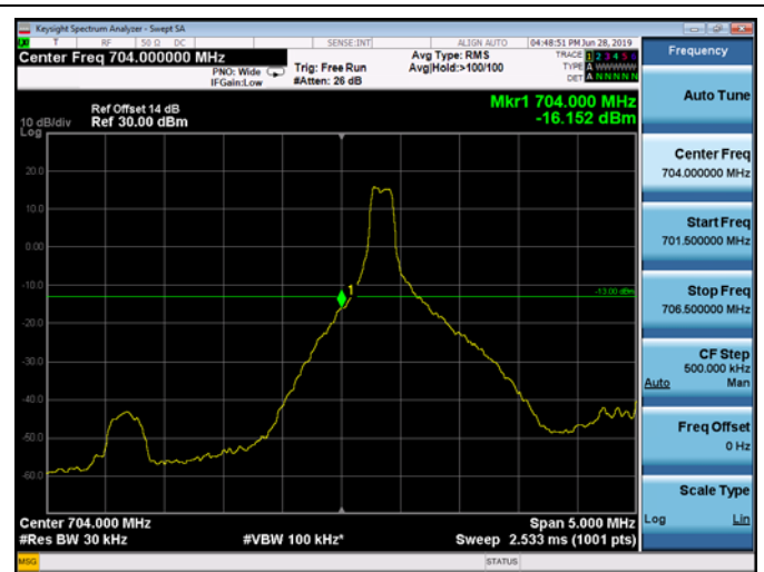
LowRange_FDD17_5MHz_706.5_fullRB _Low_Q16
