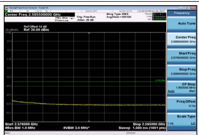
HighRange_FDD07_15MHz_2562.5_OneRB_high_Q16
