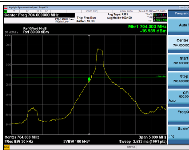
LowRange_FDD17_5MHz_706.5_fullRB _Low_QPSK
