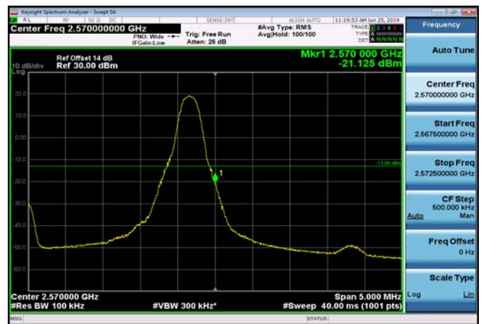
HighRange_FDD07_5MHz_2567.5_OneRB _high_Q16
