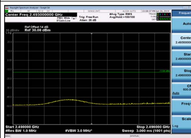
LowRange_FDD07_20MHz_2510_fullIRB_Low_Q16
