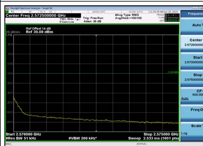
FDD07_15MHz_2562.5_Q16_OneRB_high_ExtraBands_Range_2570~2575
