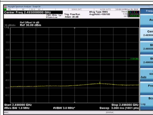
LowRange_FDD07_15MHz_2507.5_fullRB _Low_Q16
