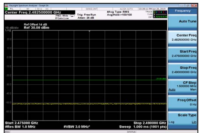
FDD07_15MHz_2562.5_QPSK_fullRB _ExtraBands_Range_2475~2490
