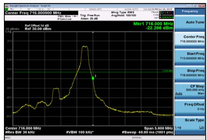
HighRange_FDD12_1.4MHz_715.3_OneRB _high_Q16
