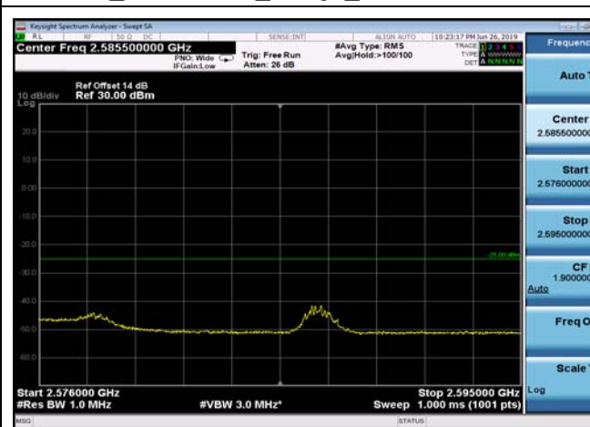
FDD07_10MHz_2565_Q16_OneRB_high _ExtraBands_Range_2576~2595
