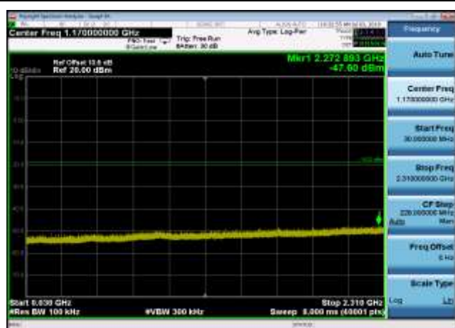
,Plot 3,30MHz~2310MHz-802.11g,2462MHz
