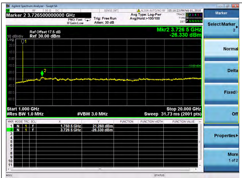
(Plot N3.1, HSUPA1700MHz, Channel = 1513, 1GHz to 20GHz)
