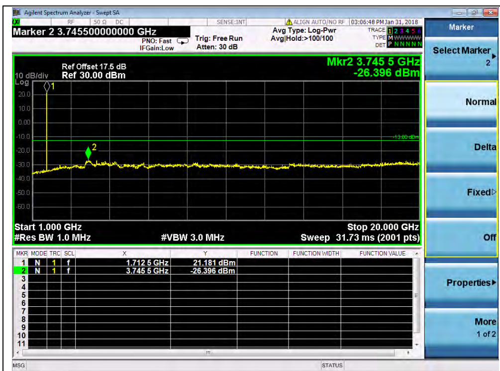
(Plot H1.1, WCDMA1700MHz, Channel = 1312, 1GHz to 20GHz)
