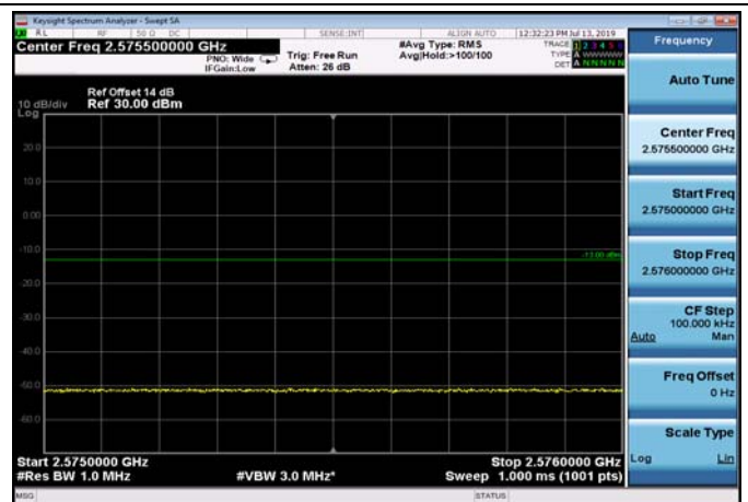
LowRange_FDD07_15MHz_2507.5_OneRB _low_QPSK
