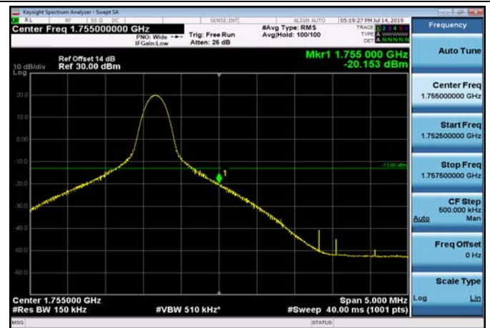
HighRange_FDD04_15MHz_1747.5_fullRB _High_Q16
