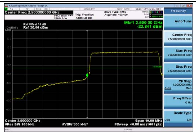
LowRange_FDD07_5MHz_2502.5_fullRB _Low_QPSK
