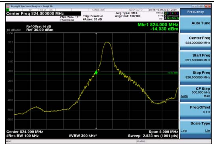
LowRange_FDD05_5MHz_826.5_OneRB _low_Q16
