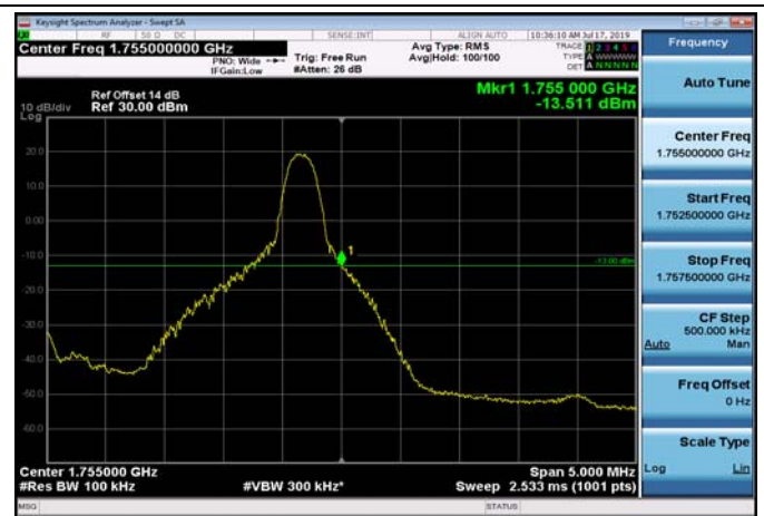
HighRange_FDD04_5MHz_1752.5_OneRB _high_Q16
