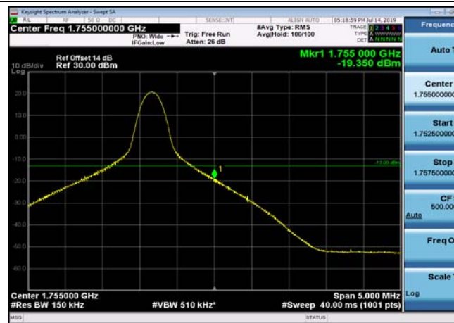
HighRange_FDD04_15MHz_1747.5_fullRB _High_QPSK
