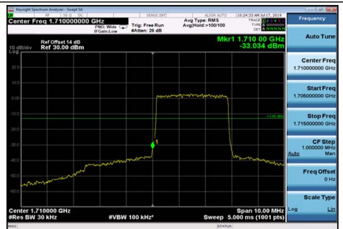
LowRange_FDD04_5MHz_1712.5_OneRB _low_Q16
