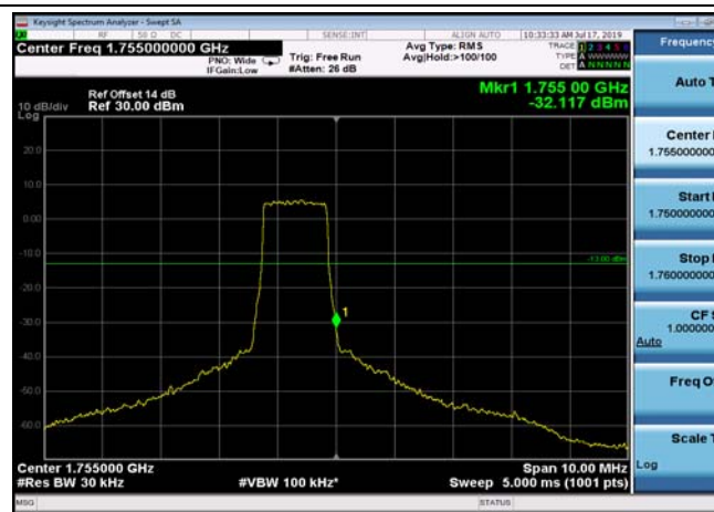
HighRange_FDD04_1.4MHz_1754.3 _fullRB_High_QPSK
