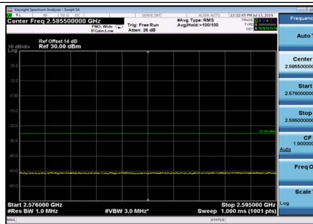
FDD07_15MHz_2507.5_QPSK_OneRB_high _ExtraBands_Range_2576~2595
