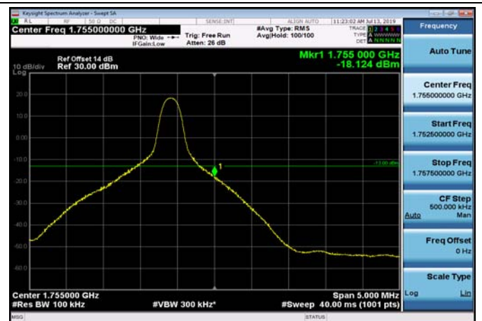
HighRange_FDD04_10MHz_1750_fullRB _High_Q16
