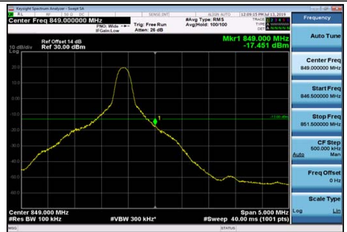
HighRange_FDD05_10MHz_844_fullRB _High_Q16
