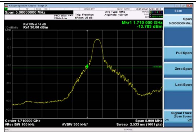
LowRange_FDD04_5MHz_1712.5_OneRB _low_Q16
