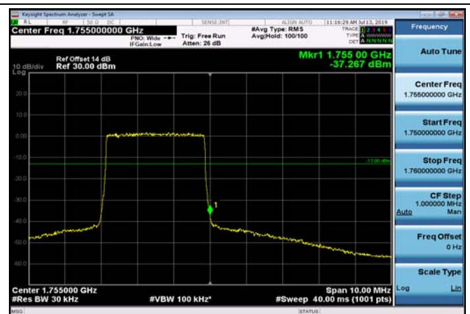
HighRange_FDD04_5MHz_1752.5_OneRB _high_Q16
