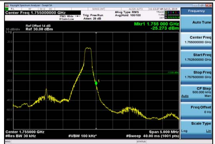
HighRange_FDD04_3MHz_1753.5_fullRB _High_Q16
