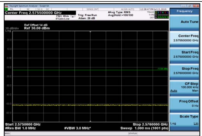
FDD07_20MHz_2510_QPSK_OneRB_high_ExtraBands_Range_2575~2576
