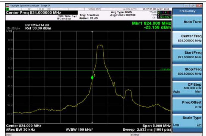
LowRange_FDD05_1.4MHz_824.7_fullRB _Low_Q16
