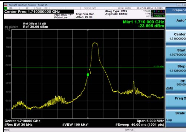
LowRange_FDD04_3MHz_1711.5_fullRB _Low_QPSK
