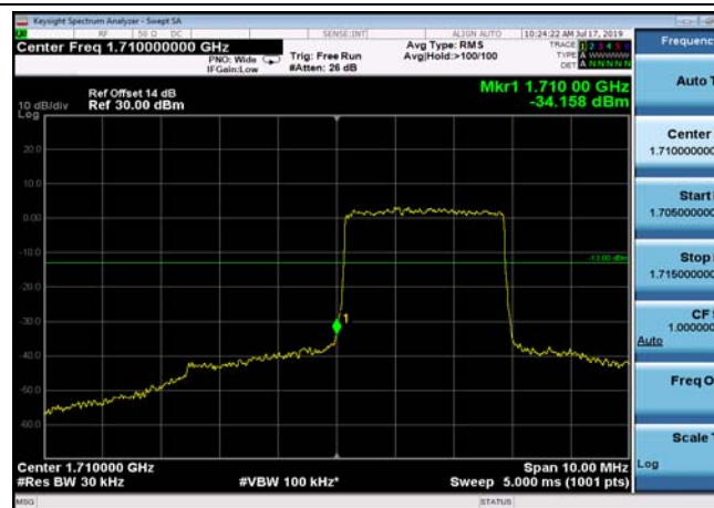
LowRange_FDD04_5MHz_1712.5_OneRB _low_QPSK
