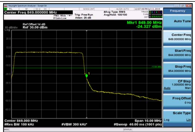
HighRange_FDD05_5MHz_846.5_fullRB _High_Q16
