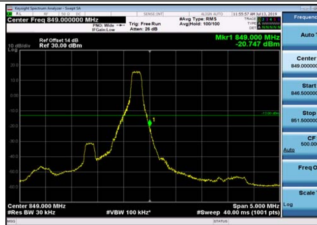
HighRange_FDD05_1.4MHz_848.3_fullRB _High_QPSK
