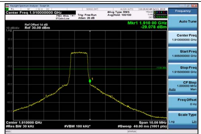
HighRange_FDD02_1.4MHz_1909.3 _fullRB_High_Q16
