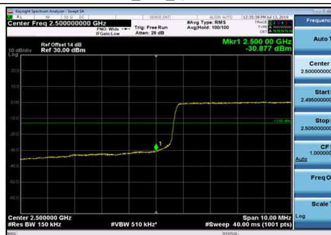
LowRange_FDD07_15MHz_2507.5_fullRB_Low_Q16
