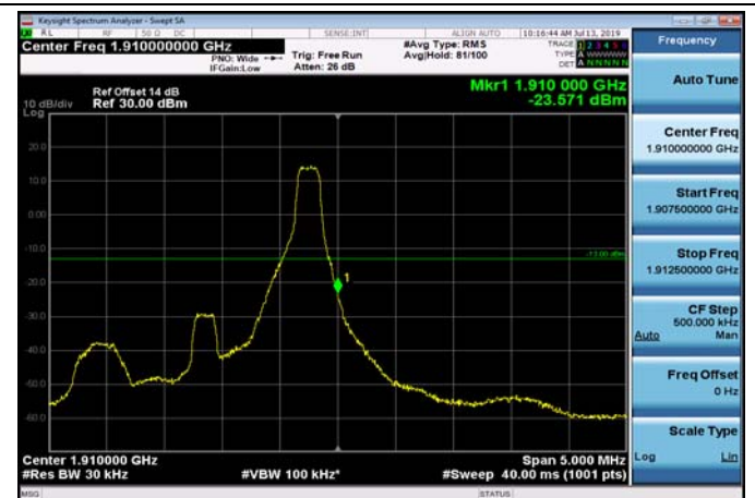
HighRange_FDD02_1.4MHz_1909.3 _fullRB_High_Q16
