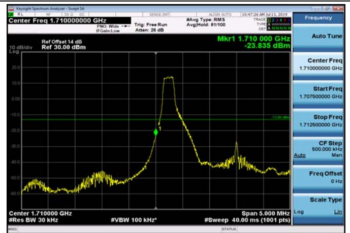
LowRange_FDD04_3MHz_1711.5_fullRB _Low_Q16
