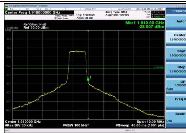
HighRange_FDD02_1.4MHz_1909.3 _fullRB_High_QPSK
