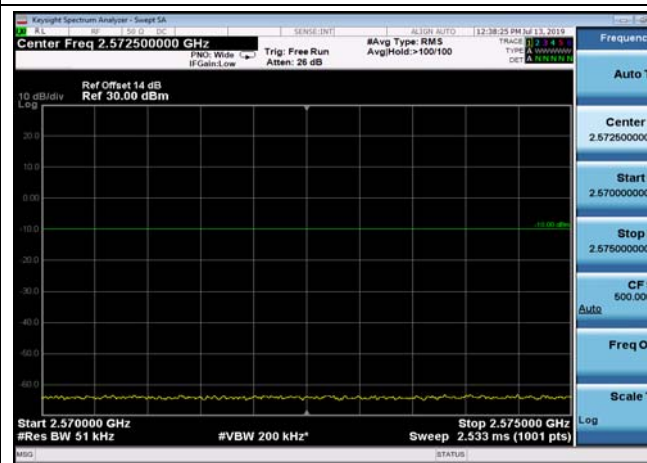
FDD07_20MHz_2510_QPSK_OneRB_high_ExtraBands_Range_2570~2575
