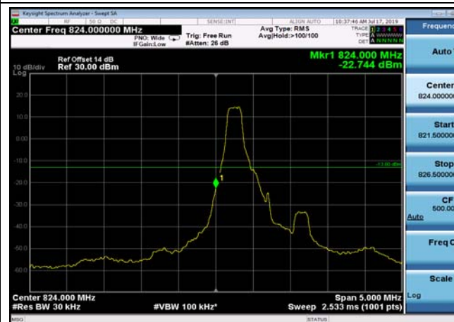
LowRange_FDD05_1.4MHz_824.7_fullRB _Low_QPSK
