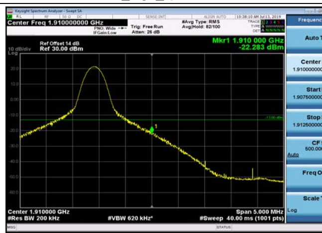
HighRange_FDD02_20MHz_1900_OneRB _high_QPSK
