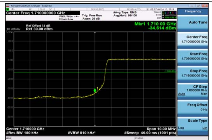
LowRange_FDD04_20MHz_1720_OneRB _low_Q16
