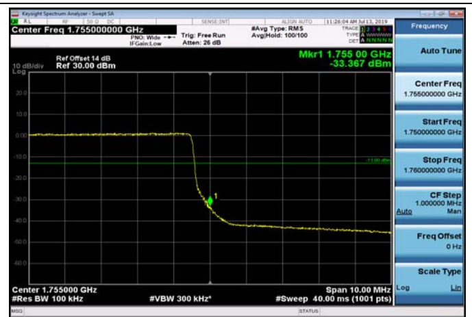
HighRange_FDD04_10MHz_1750_fullRB _High_Q16
