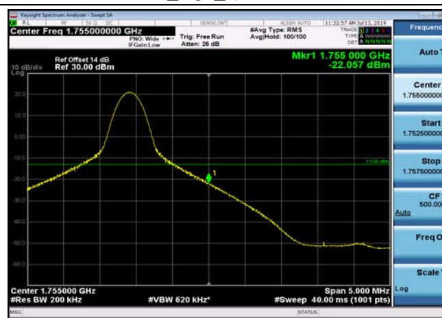
HighRange_FDD04_20MHz_1745_OneRB _high_QPSK
