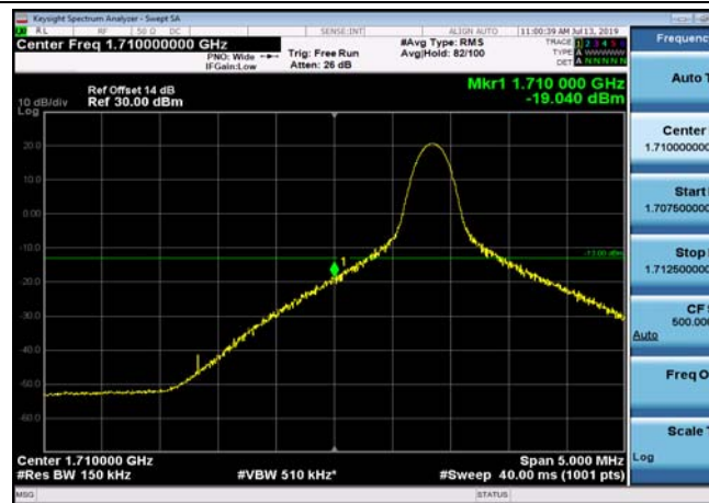
LowRange_FDD04_15MHz_1717.5_fullRB _Low_QPSK
