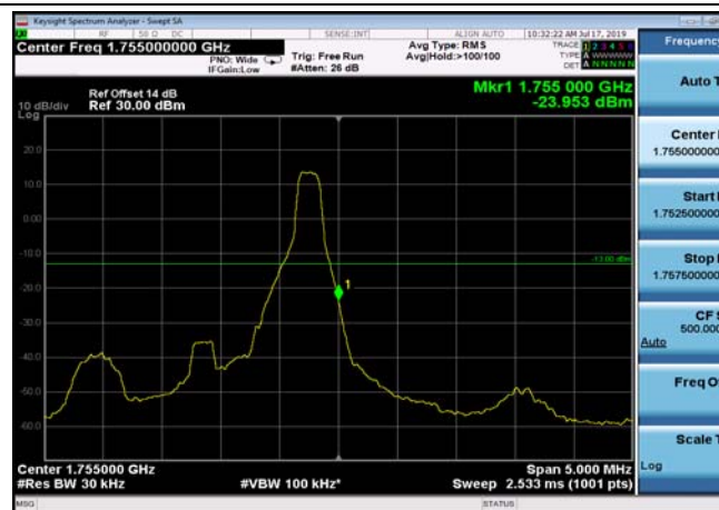
HighRange_FDD04_1.4MHz_1754.3 _fullRB_High_QPSK
