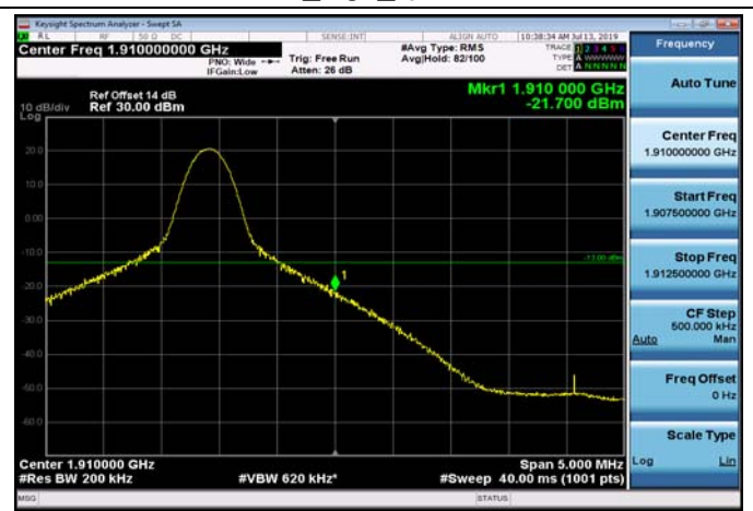
HighRange_FDD02_20MHz_1900_OneRB _high_Q16
