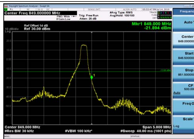
HighRange_FDD05_3MHz_847.5_OneRB _high_QPSK
