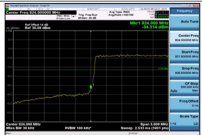
LowRange_FDD05_5MHz_826.5_OneRB _low_Q16
