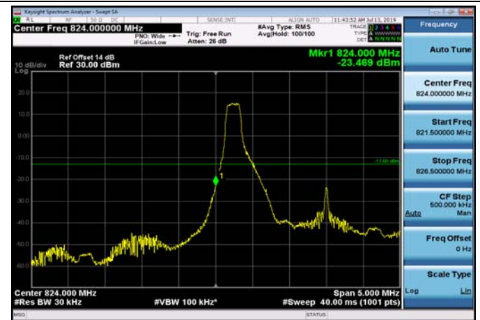
LowRange_FDD05_3MHz_825.5_fullRB _Low_Q16
