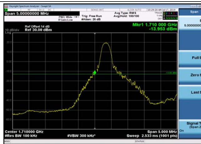
LowRange_FDD04_5MHz_1712.5_OneRB _low_QPSK
