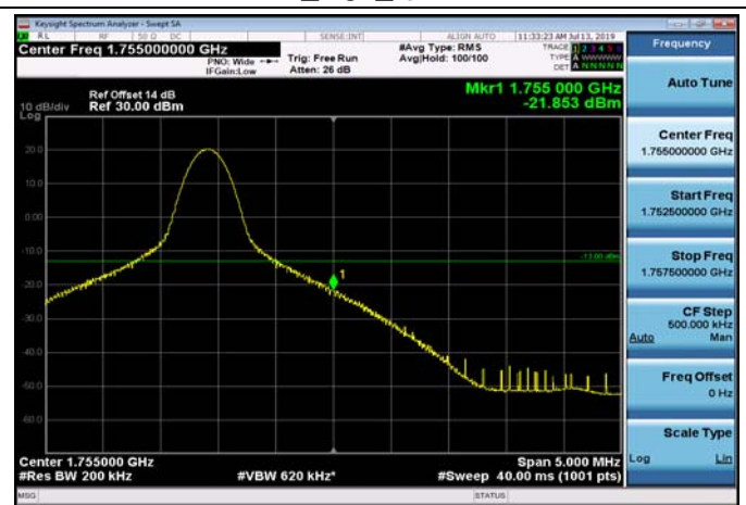
HighRange_FDD04_20MHz_1745_OneRB _high_Q16
