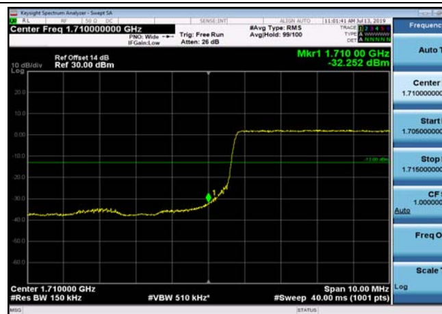
LowRange_FDD04_20MHz_1720_OneRB _low_QPSK
