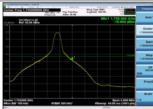
HighRange_FDD04_10MHz_1750_fullRB _High_QPSK
