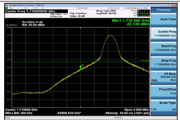
LowRange_FDD04_20MHz_1720_OneRB _low_Q16
