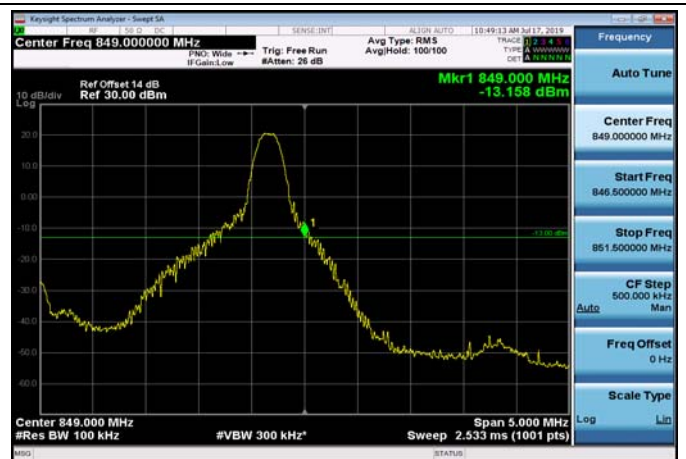
HighRange_FDD05_5MHz_846.5_fullRB _High_Q16
