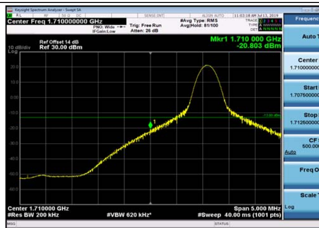
LowRange_FDD04_20MHz_1720_OneRB _low_QPSK
