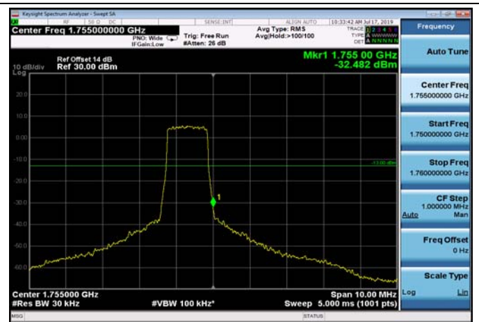
HighRange_FDD04_1.4MHz_1754.3 _fullRB_High_Q16
