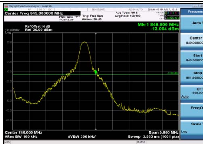
HighRange_FDD05_5MHz_846.5_fullRB _High_QPSK
