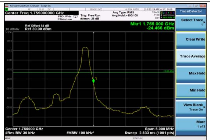
HighRange_FDD04_1.4MHz_1754.3 _fullRB_High_Q16
