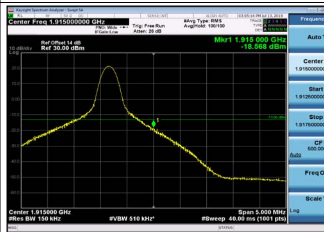
HighRange_FDD25_15MHz_1907.5_OneRB _high_QPSK
