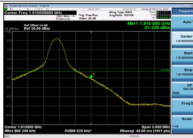
HighRange_FDD25_20MHz_1905_fullRB _High_QPSK
