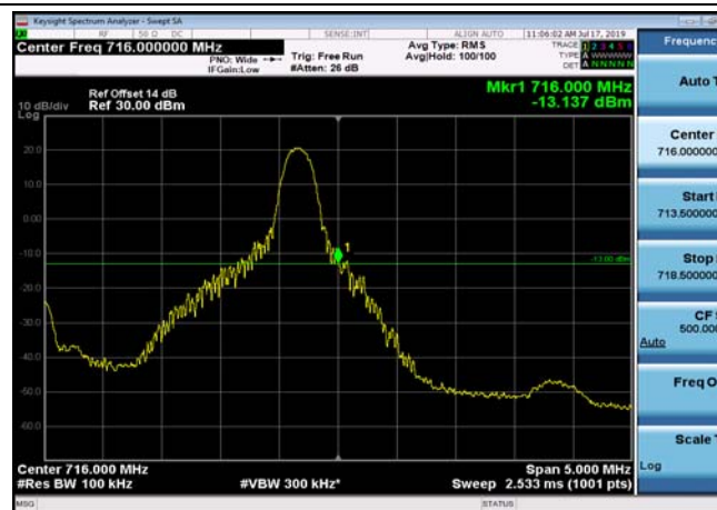
HighRange_FDD12_5MHz_713.5_fullRB _High_QPSK
