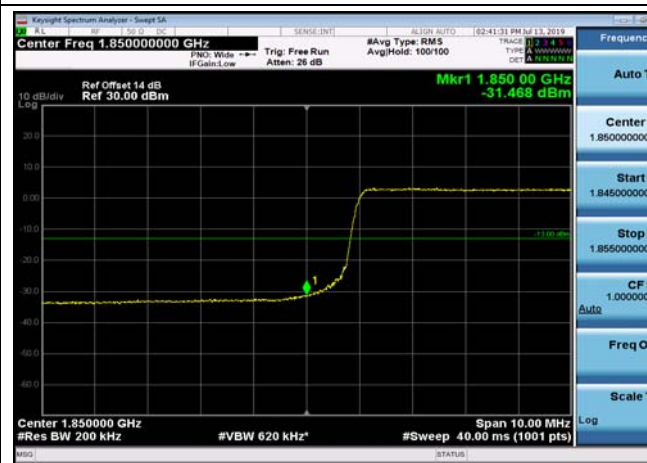
LowRange_FDD25_20MHz_1860_fullRB _Low_QPSK
