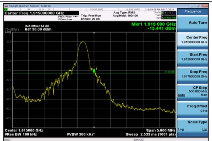
HighRange_FDD25_5MHz_1912.5_fullRB _High_Q16
