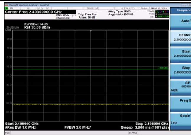
HighRange_FDD07_20MHz_2560_fullRB _High_Q16
