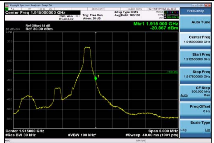
HighRange_FDD25_1.4MHz_1914.3 _fullRB_High_Q16
