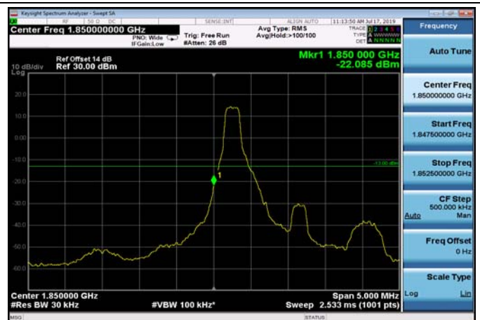
LowRange_FDD25_1.4MHz_1850.7_fullRB _Low_Q16
