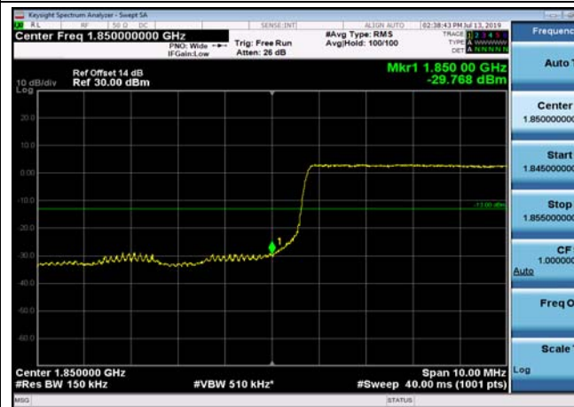
LowRange_FDD25_20MHz_1860_OneRB _low_QPSK
