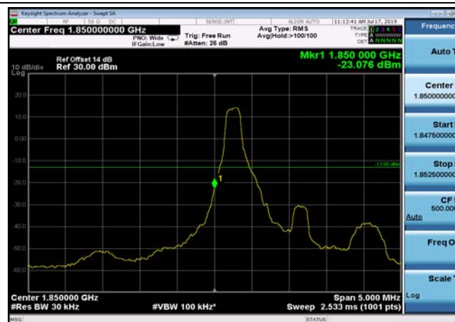
LowRange_FDD25_1.4MHz_1850.7_fullRB _Low_QPSK
