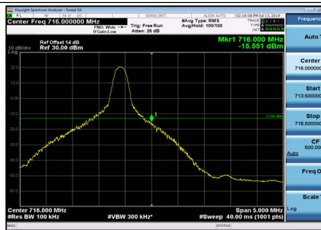
HighRange_FDD17_10MHz_711_OneRB _high_QPSK
