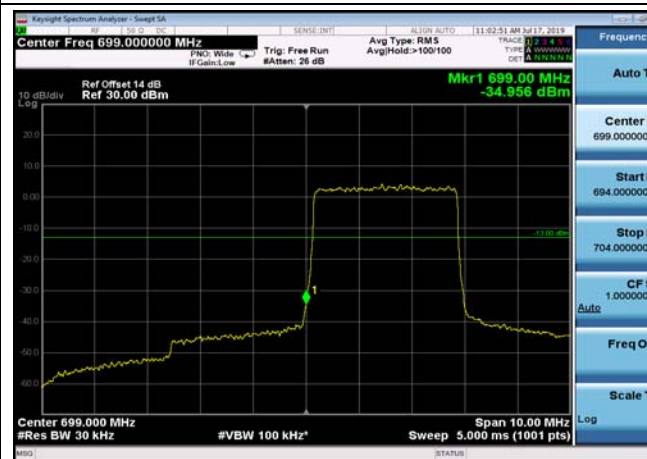
LowRange_FDD12_5MHz_701.5_OneRB _low_QPSK
