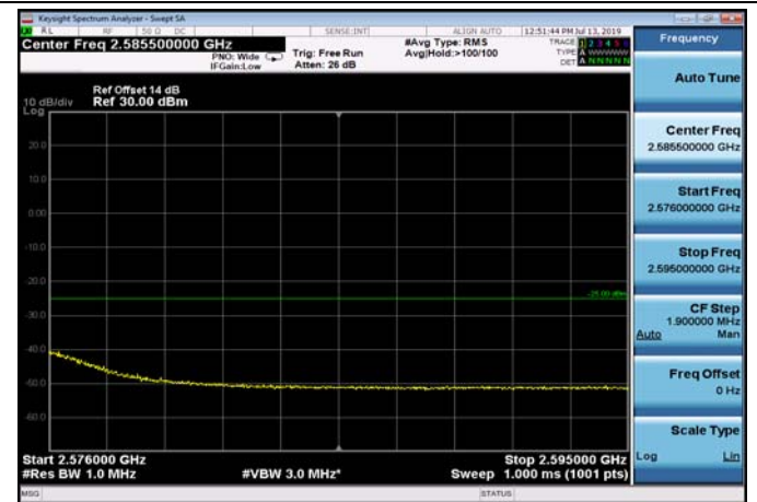
HighRange_FDD07_10MHz_2565_OneRB_high_Q16
