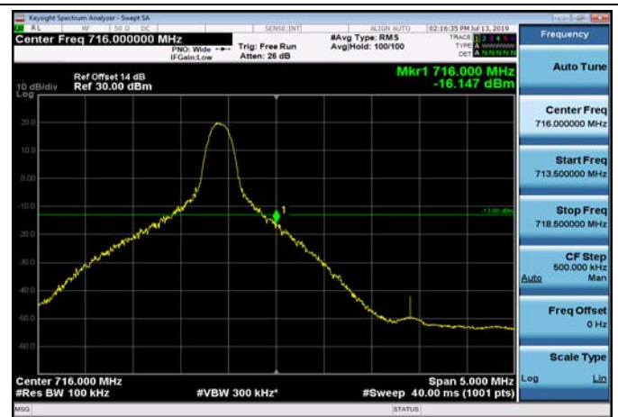
HighRange_FDD17_10MHz_711_OneRB _high_Q16
