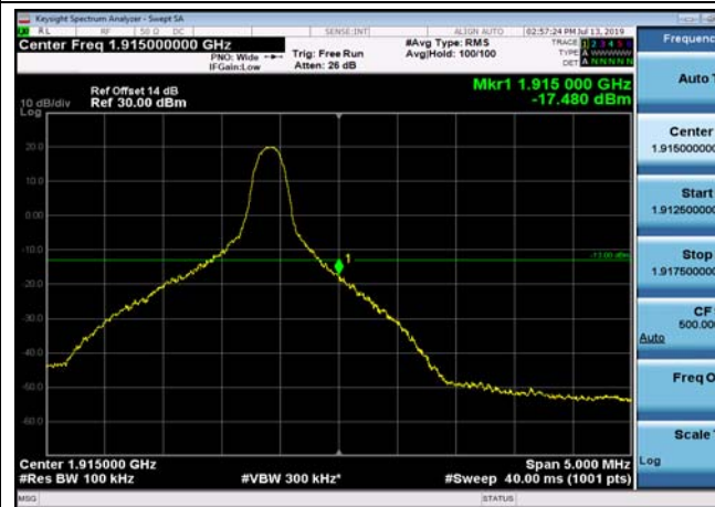
HighRange_FDD25_10MHz_1910_fullRB _High_QPSK
