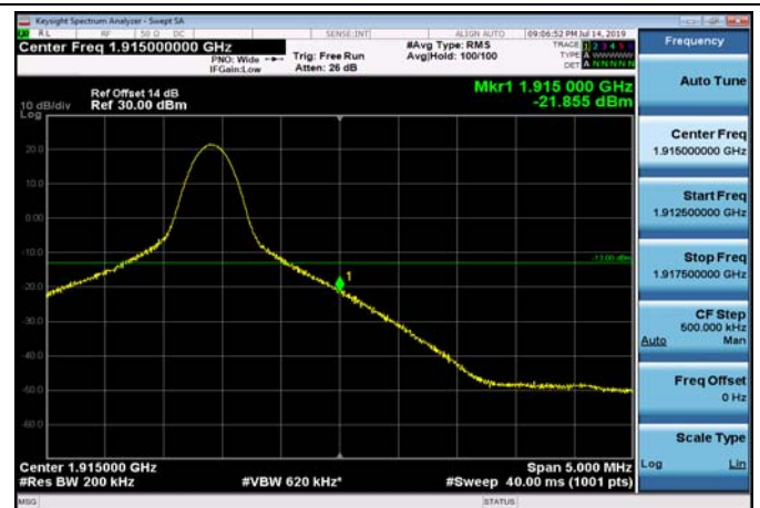
HighRange_FDD25_20MHz_1905_fullRB _High_Q16
