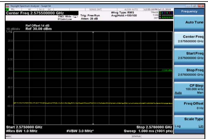
FDD07_10MHz_2565_Q16_OneRB_high_ExtraBands_Range_2575~2576
