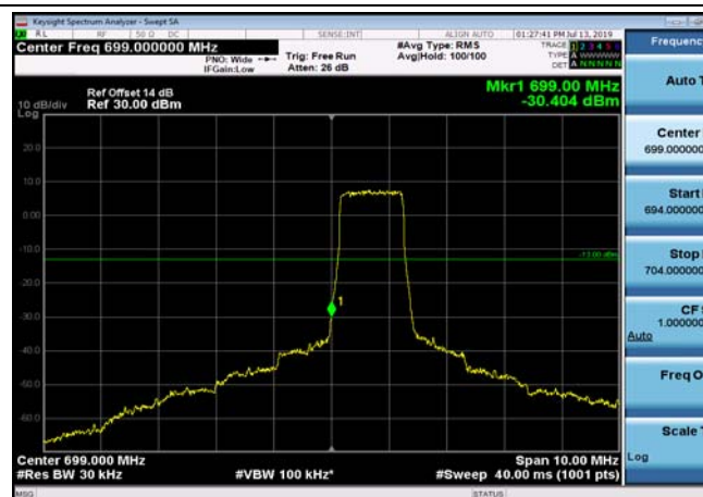
LowRange_FDD12_1.4MHz_699.7_fullRB _Low_QPSK
