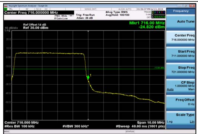
HighRange_FDD12_5MHz_713.5_fullRB _High_Q16
