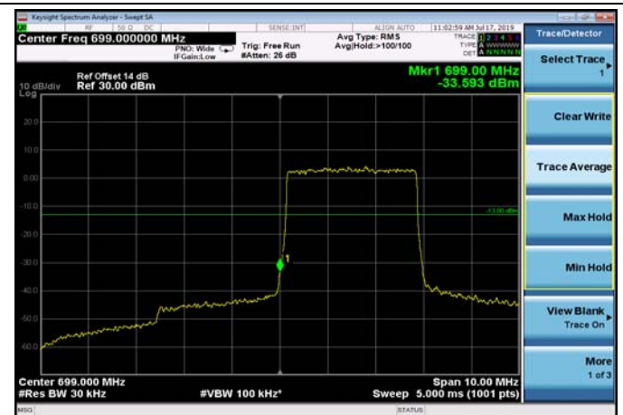
LowRange_FDD12_5MHz_701.5_OneRB _low_Q16
