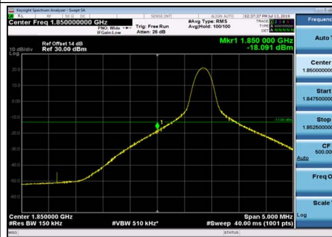
LowRange_FDD25_15MHz_1857.5_OneRB _low_QPSK
