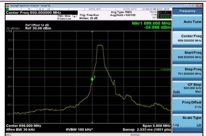
LowRange_FDD12_1.4MHz_699.7_fullRB _Low_Q16
