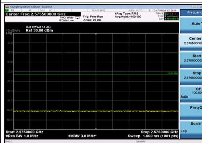
FDD07_15MHz_2562.5_QPSK_fullRB _ExtraBands_Range_2575~2576
