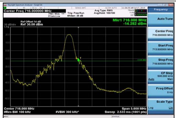
HighRange_FDD12_5MHz_713.5_fullRB _High_Q16
