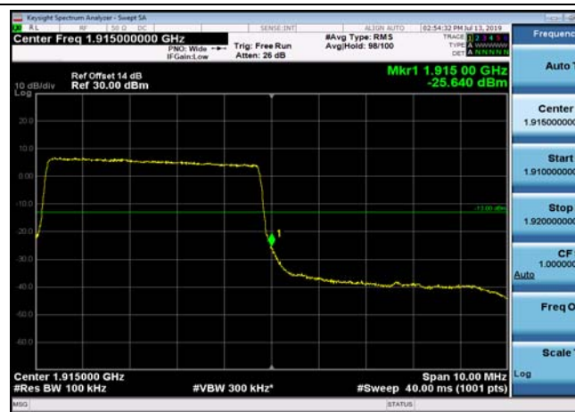
HighRange_FDD25_5MHz_1912.5_fullRB _High_QPSK
