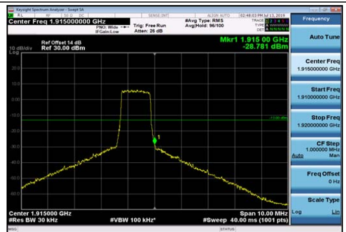
HighRange_FDD25_3MHz_1913.5_OneRB _high_Q16
