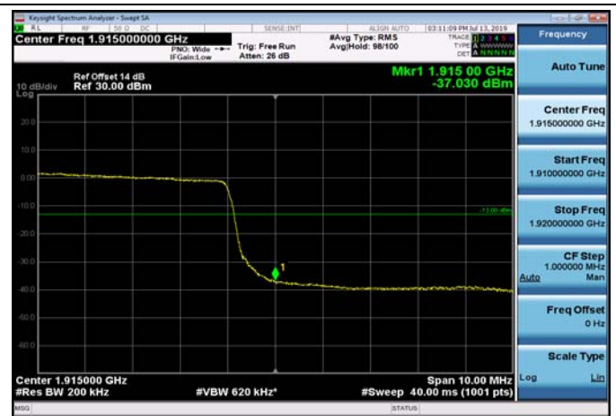
HighRange_FDD25_20MHz_1905_fullRB _High_Q16
