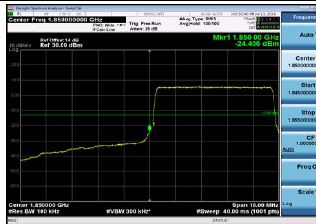
LowRange_FDD25_10MHz_1855_fullRB _Low_QPSK
