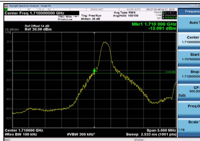
LowRange_FDD66_5MHz_1712.5_fullRB _Low_QPSK
