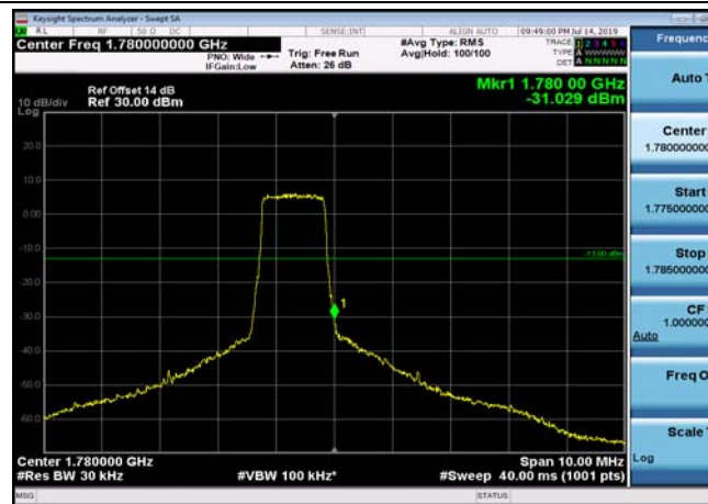
HighRange_FDD66_3MHz_1778.5_OneRB _high_QPSK
