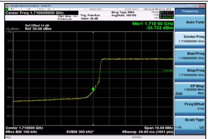
LowRange_FDD66_15MHz_1717.5_OneRB _low_Q16
