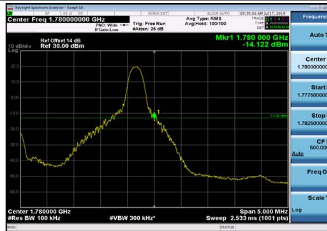
HighRange_FDD66_5MHz_1777.5_fullRB _High_QPSK
