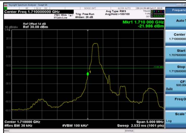
LowRange_FDD66_1.4MHz_1710.7_fullIRB _Low_QPSK
