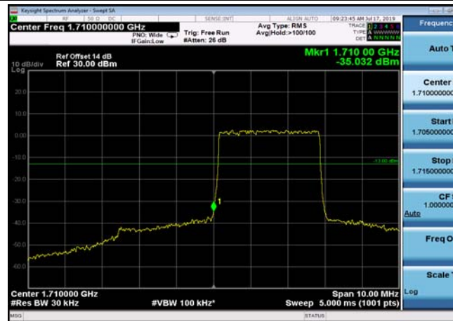
LowRange_FDD66_5MHz_1712.5_OneRB _low_QPSK
