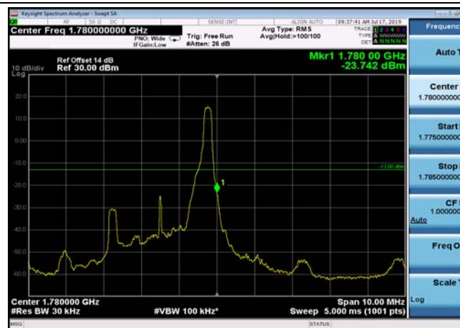
HighRange_FDD66_3MHz_1778.5_fullRB _High_QPSK
