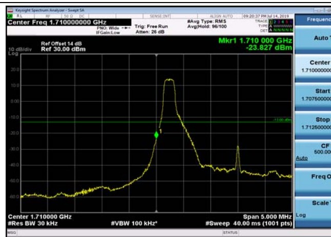
LowRange_FDD66_3MHz_1711.5_OneRB _low_QPSK
