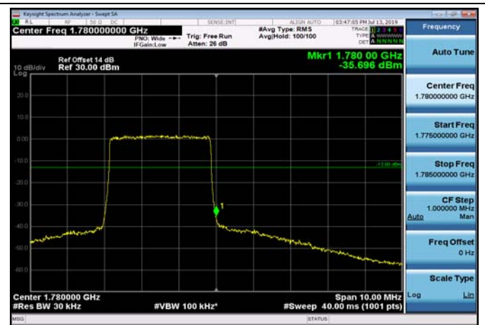
HighRange_FDD66_3MHz_1778.5_fullRB _High_Q16
