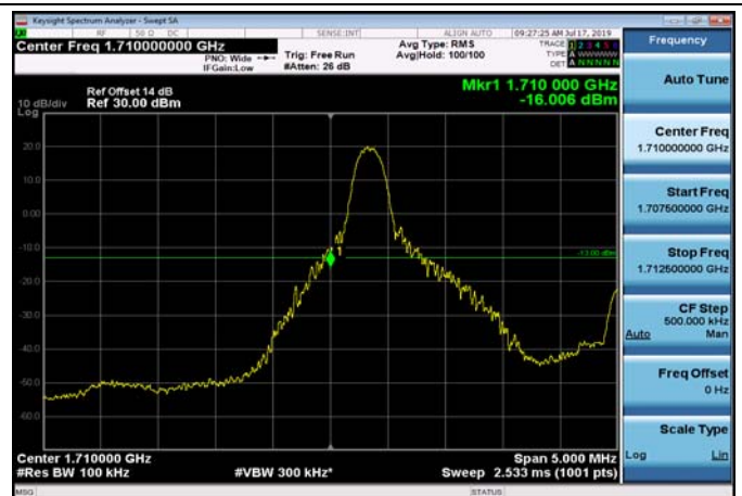
LowRange_FDD66_5MHz_1712.5_fullRB _Low_Q16
