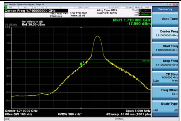
LowRange_FDD66_10MHz_1715_fullRB _Low_Q16
