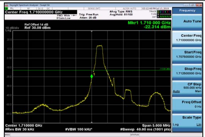
LowRange_FDD66_1.4MHz_1710.7_fullIRB _Low_Q16
