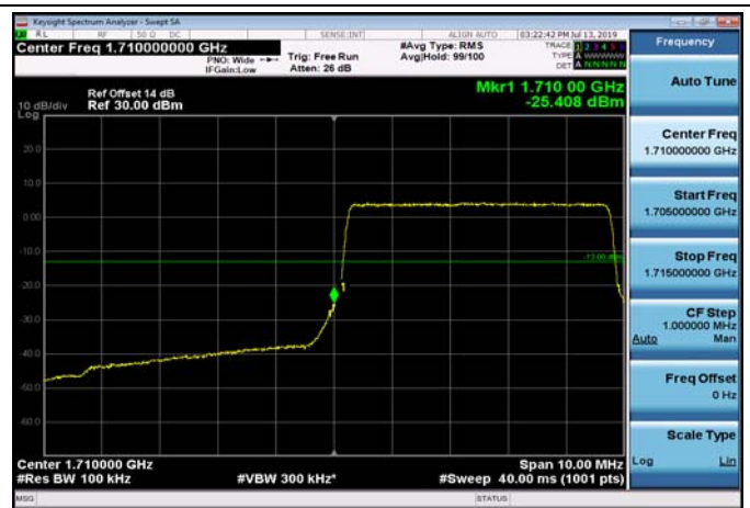
LowRange_FDD66_5MHz_1712.5_fullRB _Low_Q16
