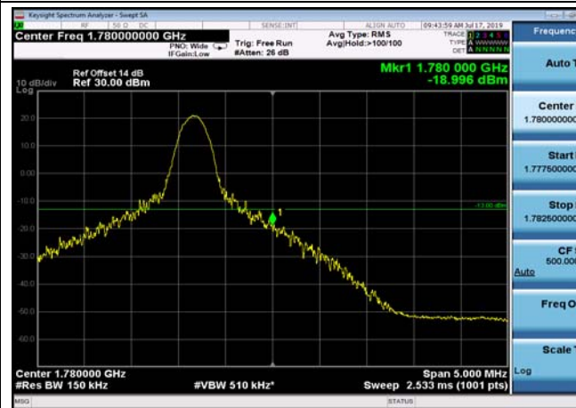
HighRange_FDD66_15MHz_1772.5_fullIRB _High_QPSK
