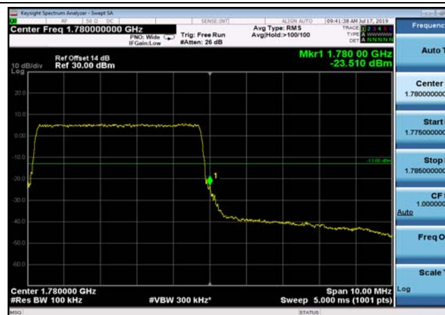
HighRange_FDD66_10MHz_1775_fullRB _High_QPSK
