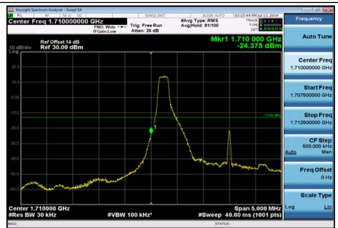
LowRange_FDD66_3MHz_1711.5_OneRB _low_Q16
