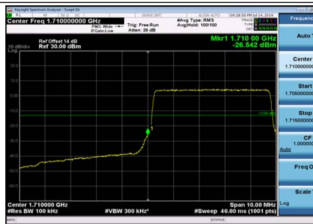
LowRange_FDD66_5MHz_1712.5_fullRB _Low_QPSK
