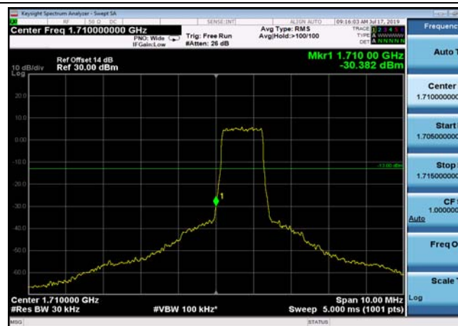
LowRange_FDD66_3MHz_1711.5_OneRB _low_QPSK
