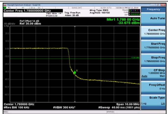
HighRange_FDD66_10MHz_1775_fullRB _High_Q16
