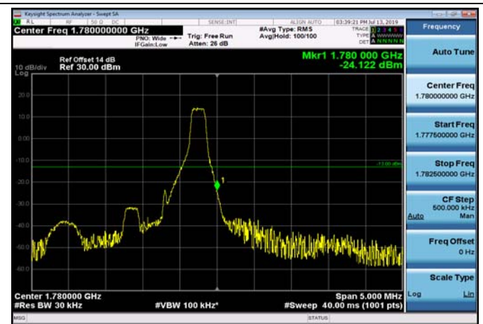
HighRange_FDD66_1.4MHz_1779.3_OneRB _high_Q16
