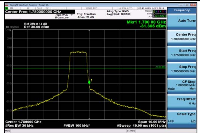
HighRange_FDD66_3MHz_1778.5_OneRB _high_Q16
