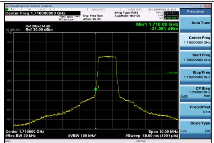
LowRange_FDD66_3MHz_1711.5_OneRB _low_Q16
