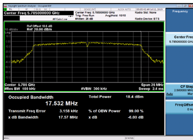
U-NII-3 6dB Bandwidth-802.11n(20MHz),5785MHz
