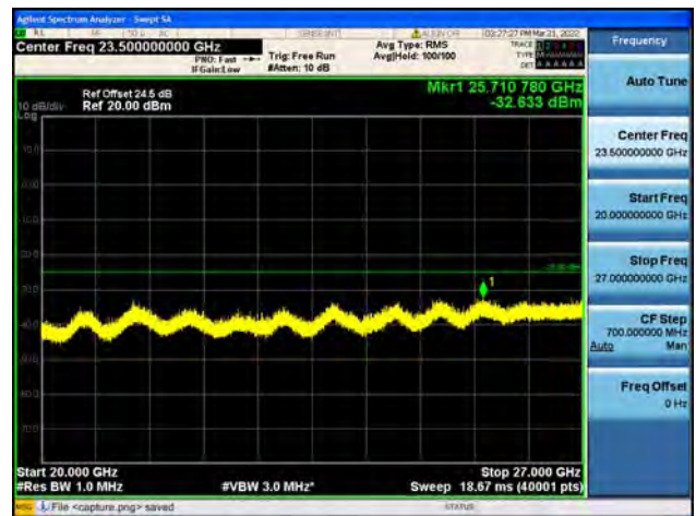
Band41-20G-27G / 15MHz / High CH / 16QAM
