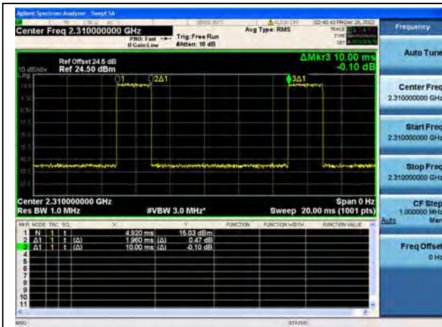
Band40-1/ Duty Cycle
