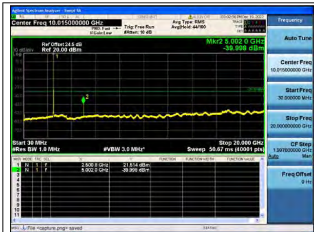
Band7-30M-20G / 20MHz / Low CH / QPSK
