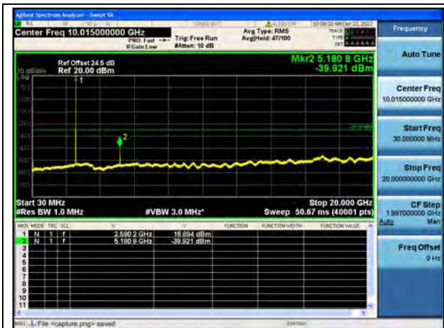
Band38-30M-20G / 10MHz / Mid CH / 16QAM
