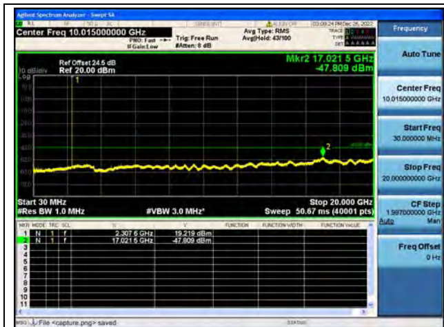
Band40-1-30M-20G / 5MHz / Mid CH / 16QAM
