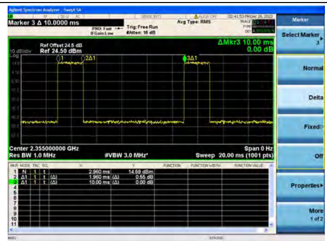
Band40-2/ Duty Cycle
