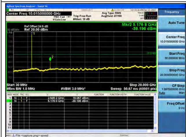
Band41-30M-20G / 10MHz / Mid CH / QPSK
