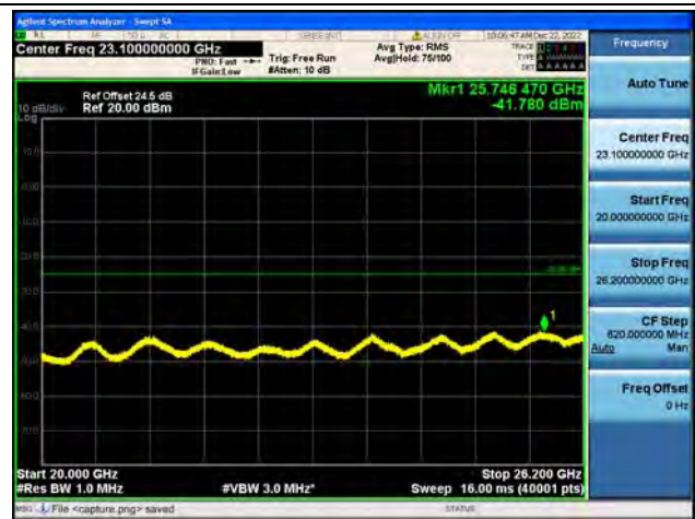
Band38-20G-26G / 5MHz / Mid CH / QPSK
