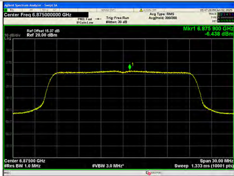
PSD NVNT ax20 6875MHz Ant2 MIMO
