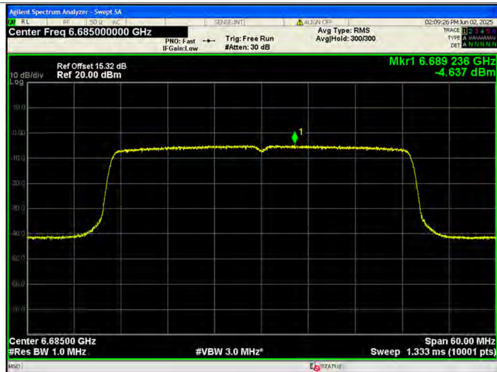
PSD NVNT ax40 6685MHz Ant2 SISO
