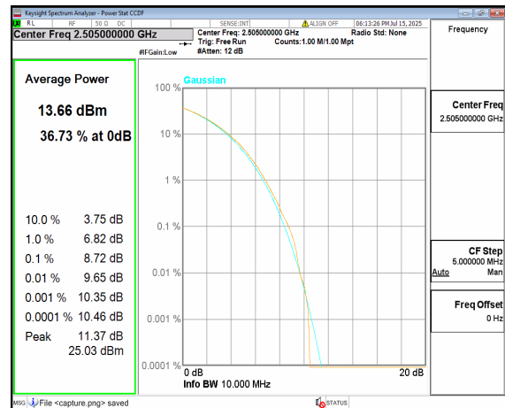
n7 10M CP-OFDM 256QAM Outer_Full Low
