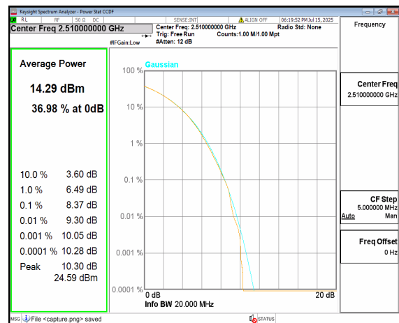
n7 20M CP-OFDM 256QAM Outer_Full Low
