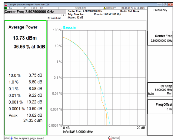
n7 5M CP-OFDM 256QAM Outer_Full Low
