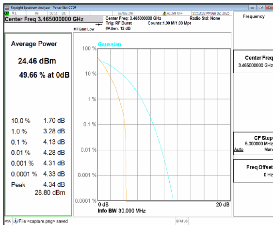
n77(3450-3550MHz) 30M DFT-s-OFDM Outer_Full Low
