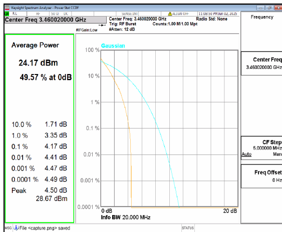
n77(3450-3550MHz) 20M DFT-s-OFDM Outer_Full Low
