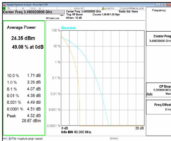
n77(3450-3550MHz) 80M DFT-s-OFDM Outer_Full Low
