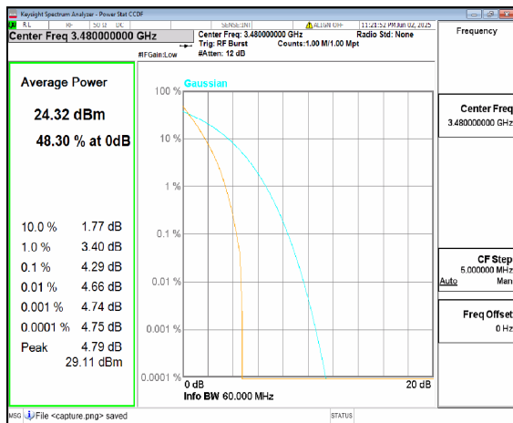
n77(3450-3550MHz) 60M DFT-s-OFDM Outer_Full Low
