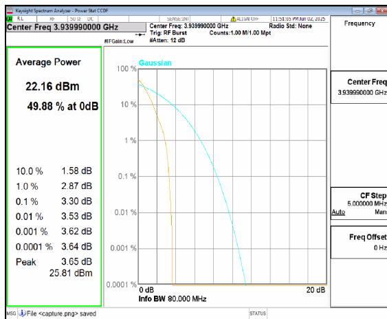
n77(3700-3980MHz) 80M DFT-s-OFDM Outer_Full High
