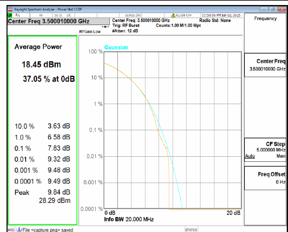
n78(3450-3550MHz) 20M CP-OFDM 256QAM Outer_Full Mid
