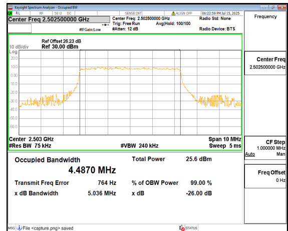
n7 5M DFT-s-OFDM 64QAM Outer_Full Low
