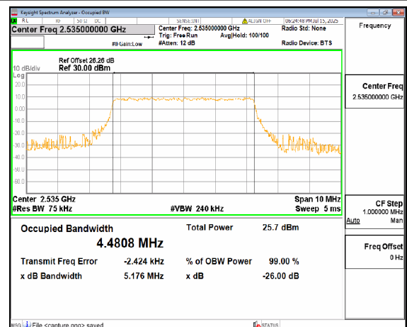
n7 5M CP-OFDM QPSK Outer_Full Mid
