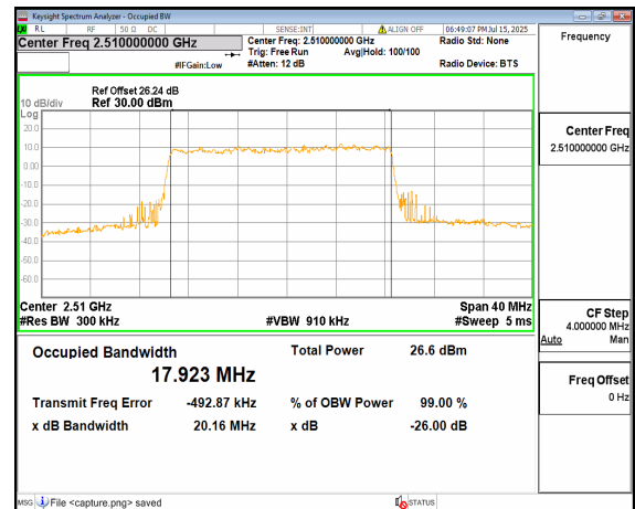
n7 20M DFT-s-OFDM 64QAM Outer_Full Low
