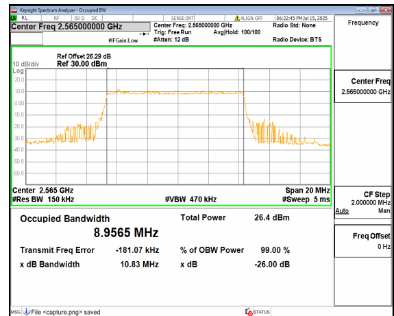
n7 10M DFT-s-OFDM 64QAM Outer_Full High
