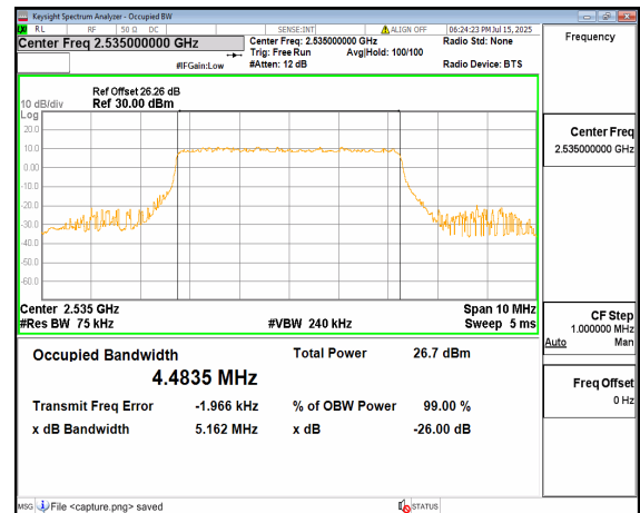
n7 5M DFT-s-OFDM 64QAM Outer_Full Mid
