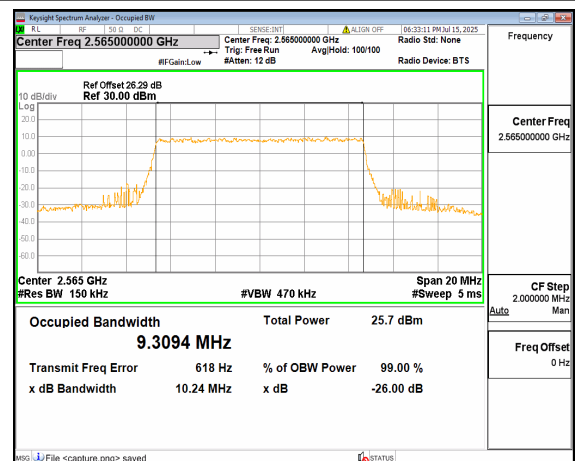
n7 10M CP-OFDM QPSK Outer_Full High
