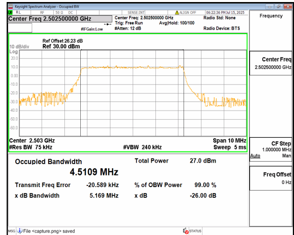
n7 5M DFT-s-OFDM QPSK Outer_Full Low
