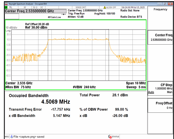
n7 5M DFT-s-OFDM QPSK Outer_Full Mid
