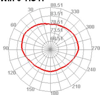
Wifi 6 TIS H
