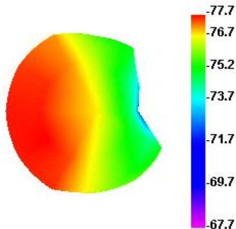
Wifi 165 TIS
