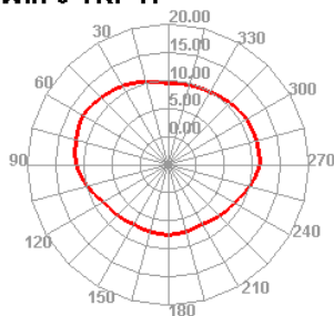
Wifi 6 TRP H
