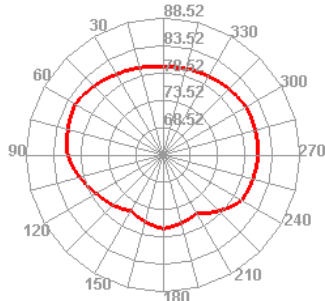
Wifi 1 TIS H
