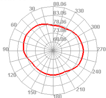
Wifi 13 TIS H
