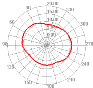
Wifi 13 TRP H
