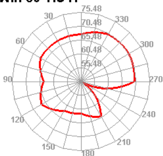
Wifi 36 TIS H
