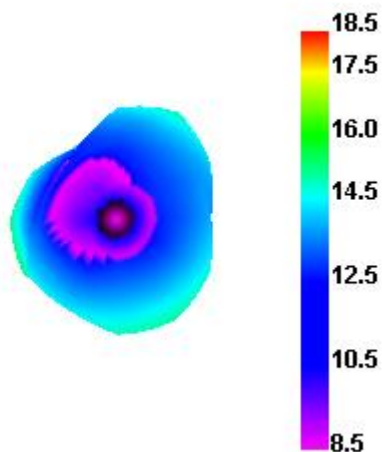
Wifi 6 TRP
