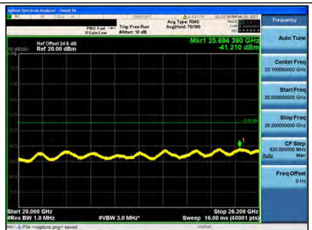
Band38-20G-26G / 10MHz / Low CH / QPSK
