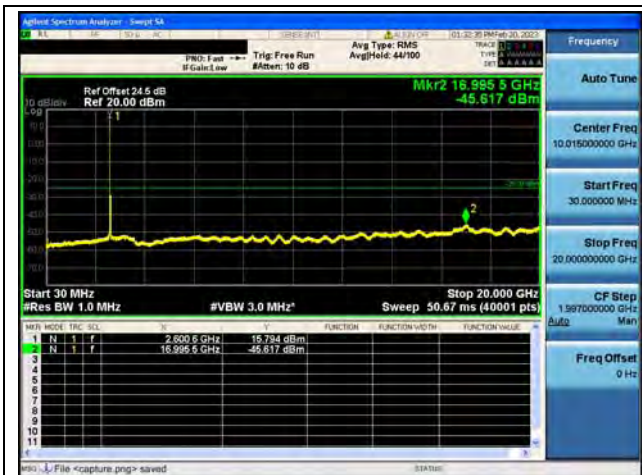
Band38-30M-20G / 20MHz / High CH / QPSK
