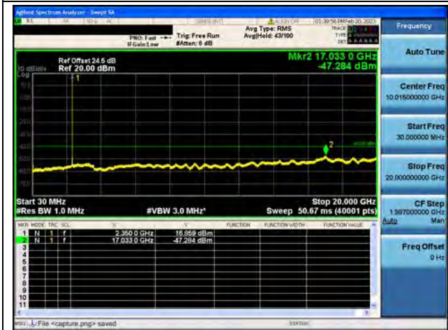
Band40-2-30M-20G / 5MHz / Low CH / 16QAM
