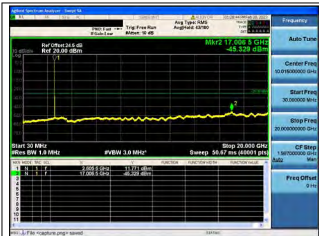
Band38-30M-20G / 15MHz / High CH / QPSK
