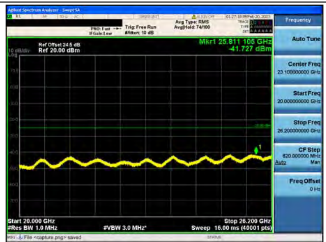
Band38-20G-26G / 15MHz / Low CH / 64QAM
