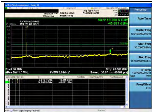
Band38-30M-20G / 10MHz / High CH / QPSK
