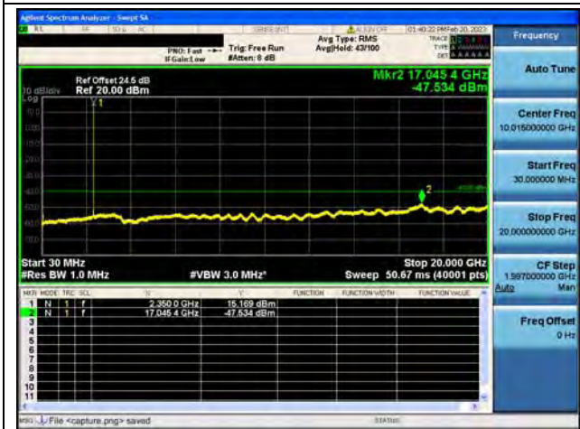
Band40-2-30M-20G / 5MHz / Low CH / 64QAM
