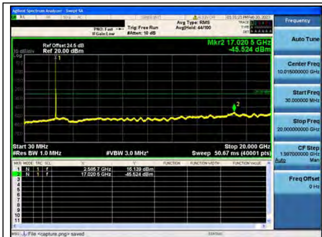
Band38-30M-20G / 20MHz / Mid CH / QPSK
