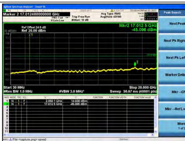
Band41(2535~2655)-30M-20G / 5MHz / High CH / 64QAM
