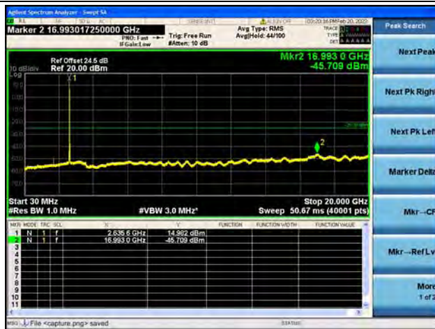
Band41(2535~2655)-30M-20G / 20MHz / High CH / 16QAM
