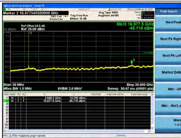
Band41(2535~2655)-30M-20G / 10MHz / Mid CH / 16QAM
