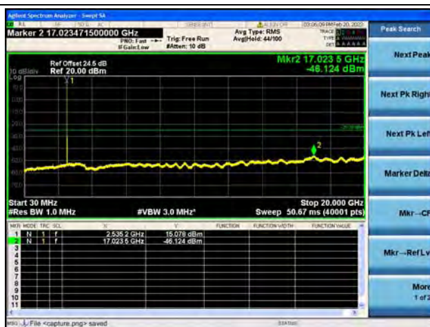
Band41(2535~2655)-30M-20G / 5MHz / Low CH / 64QAM
