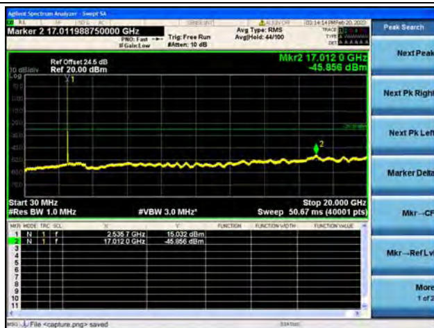
Band41(2535~2655)-30M-20G / 15MHz / Low CH / 64QAM
