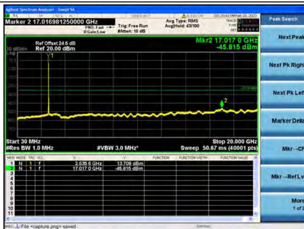
Band41(2535~2655)-30M-20G / 20MHz / High CH / 64QAM
