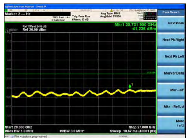
Band41(2535~2655)-20G-27G / 15MHz / Mid CH / 64QAM
