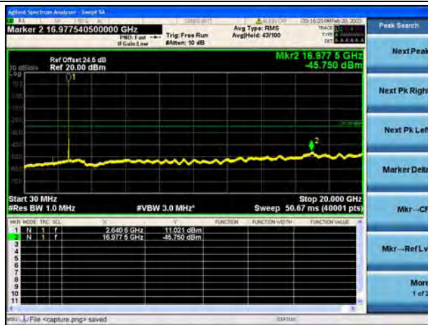
Band41(2535~2655)-30M-20G / 15MHz / High CH / 16QAM
