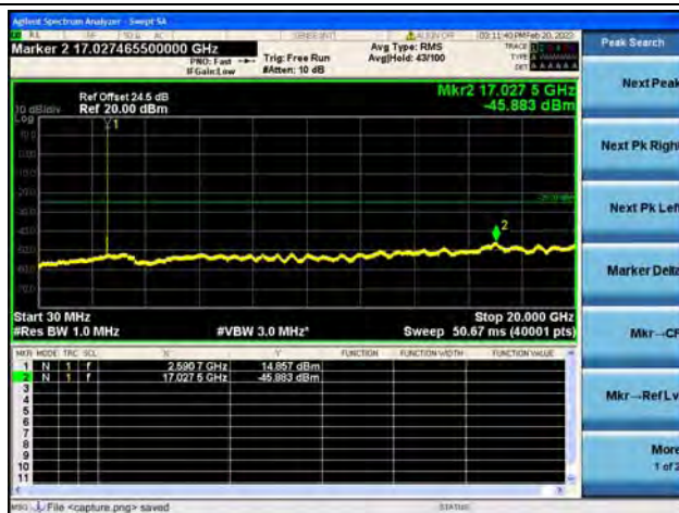
Band41(2535~2655)-30M-20G / 10MHz / Mid CH / 64QAM
