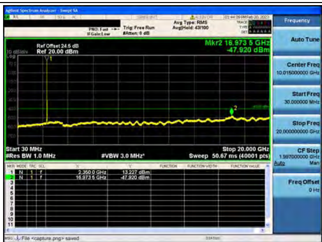
Band40-2-30M-20G / 10MHz / Mid CH / 16QAM
