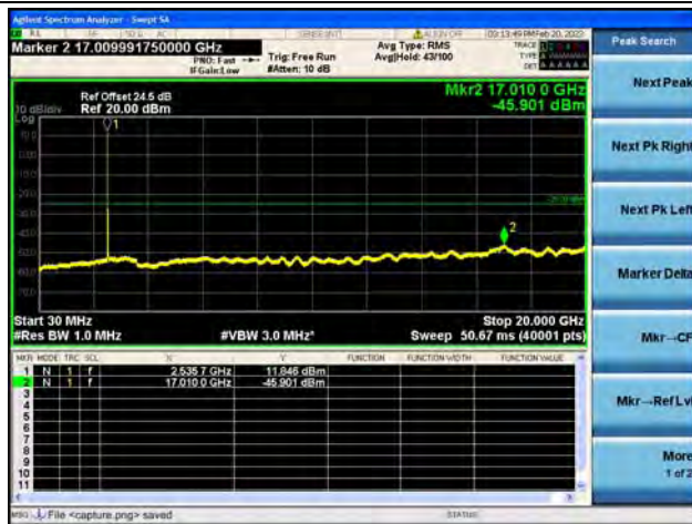
Band41(2535~2655)-30M-20G / 15MHz / Low CH / 16QAM
