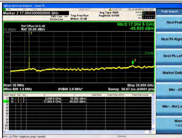
Band41(2535~2655)-30M-20G / 15MHz / High CH / 64QAM
