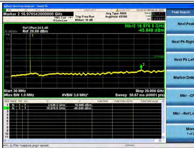
Band41(2535~2655)-30M-20G / 5MHz / Low CH / 16QAM
