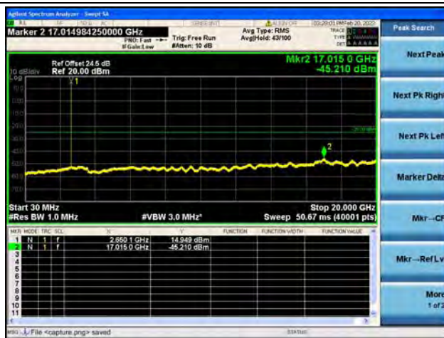
Band41(2535~2655)-30M-20G / 5MHz / High CH / 16QAM
