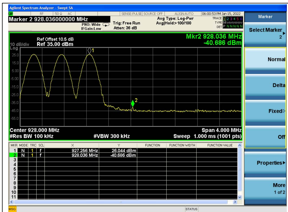
(Band edge with hopping on, Channel 50)
