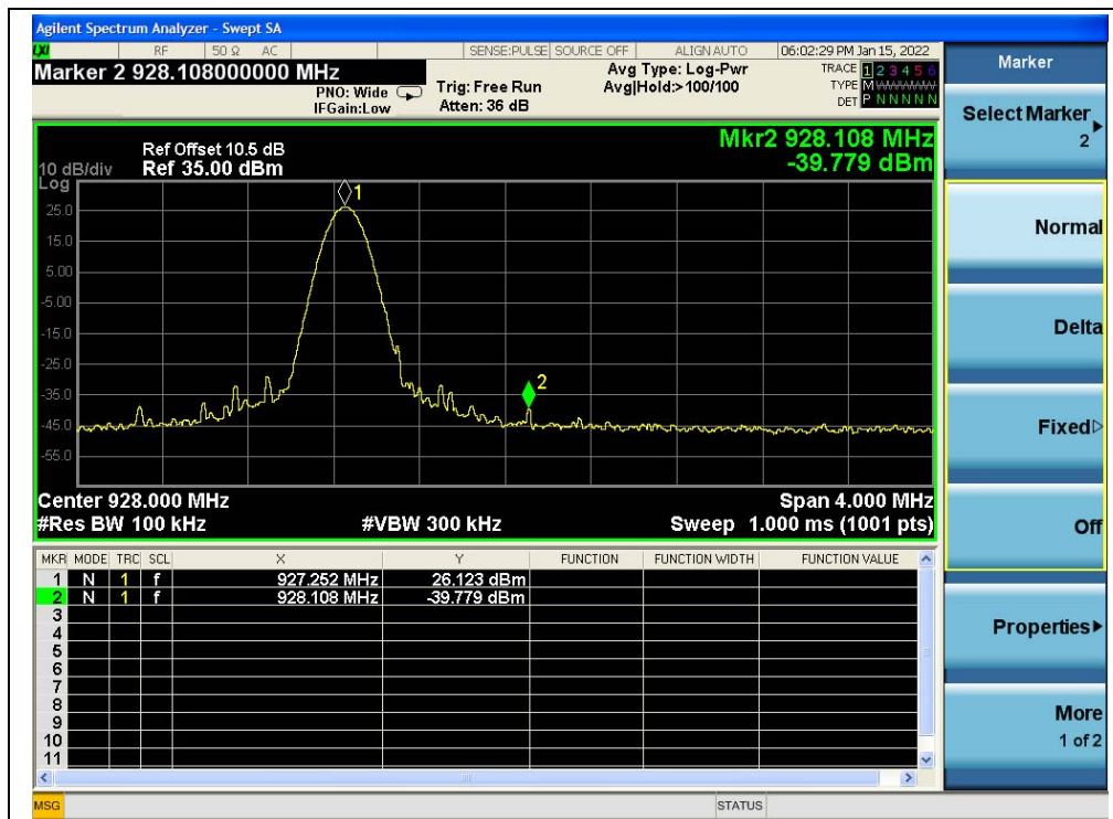
(Band edge, Channel 50)
