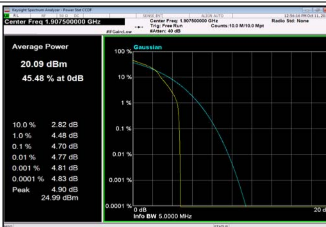
FDD02_5MHz_1907.5_OneRB_high_Q16
