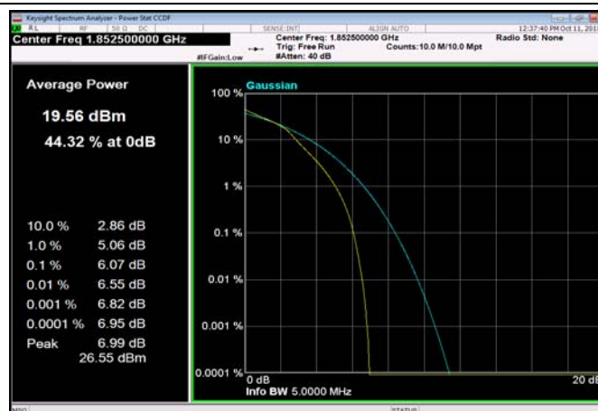
FDD02_5MHz_1852.5_fullRB_Q16
