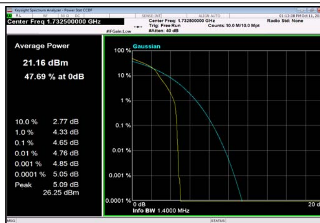
FDD04_1.4MHz_1732.5_OneRB_high_Q16
