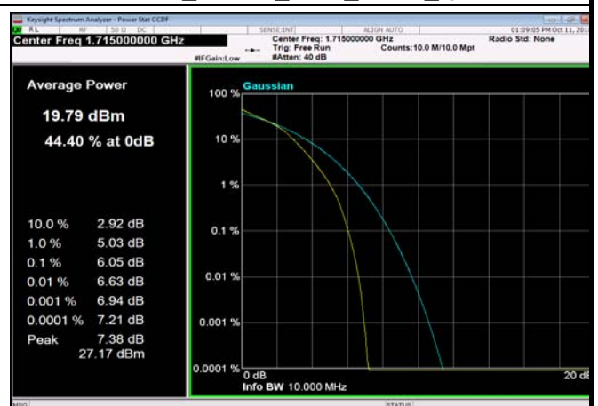
FDD04_10MHz_1715_fullRB_Q16
