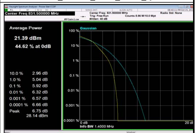
FDD26_1.4MHz_831.5_fullRB_Q16
