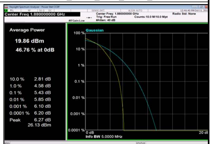
FDD02_5MHz_1880_fullRB_Q16
