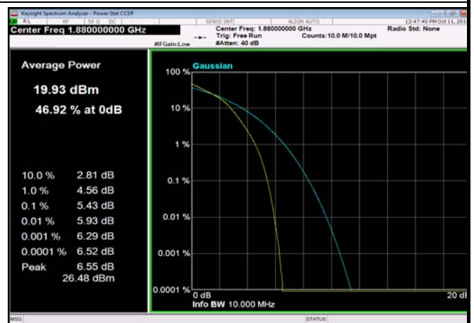
FDD02_15MHz_1880_fullRB_Q16
