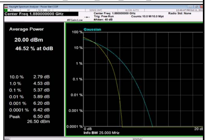
FDD02_20MHz_1880_fullRB_Q16
