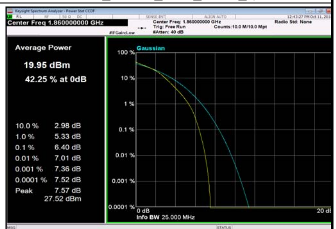
FDD02_20MHz_1860_fullRB_Q16
