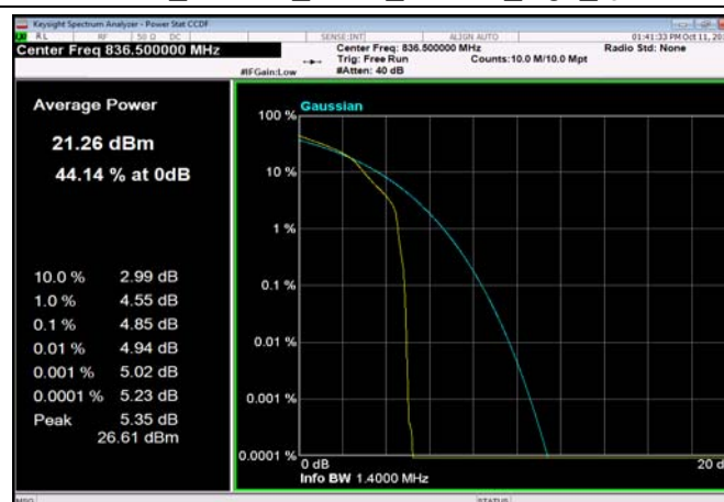
FDD05_1.4MHz_836.5_OneRB_high_Q16
