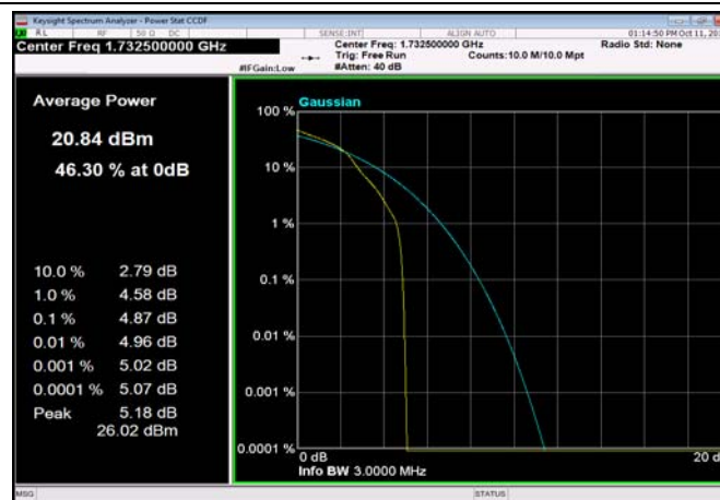
FDD04_5MHz_1732.5_OneRB_high_Q16
