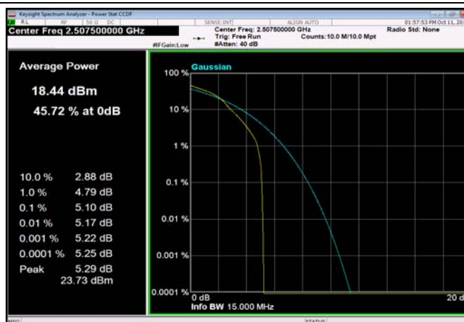
FDD07_15MHz_2507.5_OneRB_high_Q16
