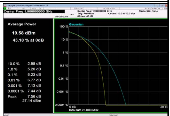
FDD02_20MHz_1900_fullRB_Q16
