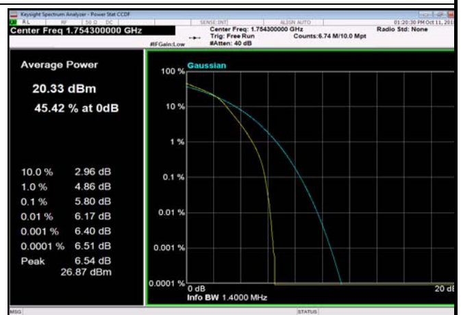
FDD04_1.4MHz_1754.3_fullRB_Q16
