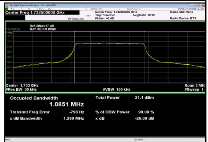
FDD04_MidRange_3MHz_1732.5MHz_Q16
