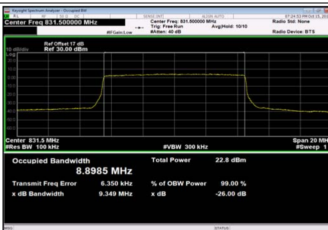
FDD26_MidRange_10MHz_831.5MHz_QPSK
