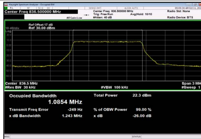
FDD05_MidRange_3_836.5_QPSK
