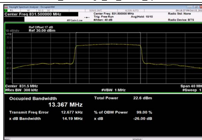
FDD26_MidRange_15_831.5_QPSK
