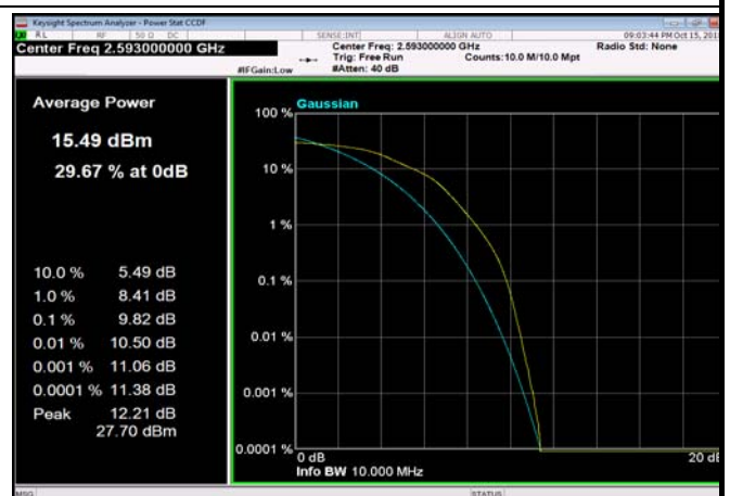
TDD41_10MHz_2593_fullRB_Q16
