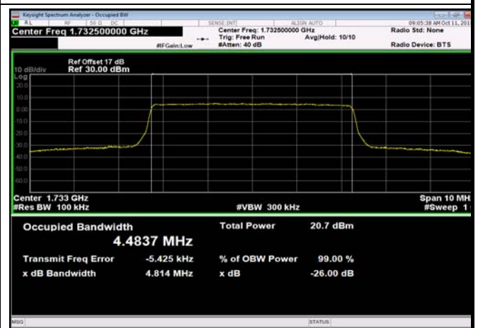
FDD04_MidRange_5MHz_1732.5MHz_Q16
