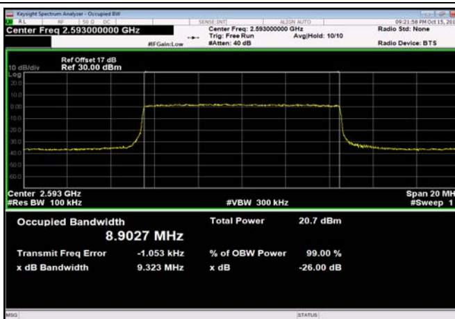
TDD41_MidRange_15_2593_QPSK
