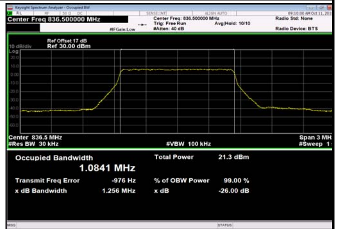
FDD05_MidRange_3_836.5_Q16
