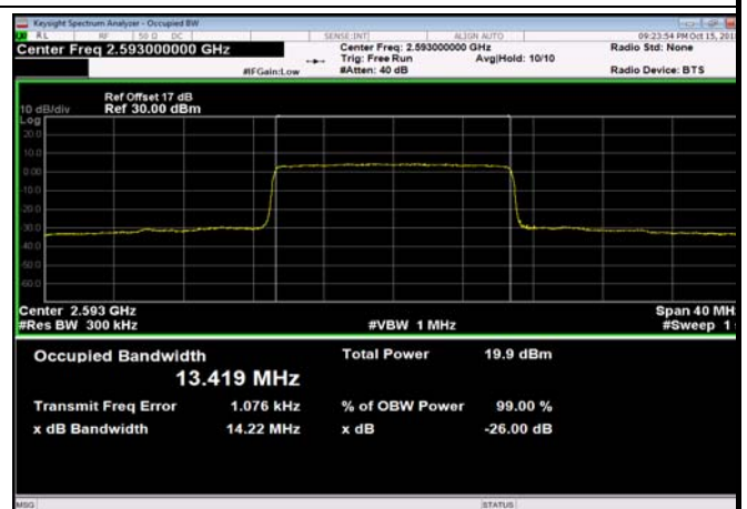
TDD41_MidRange_15_2593_Q16
