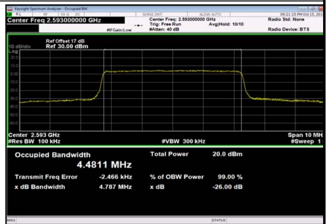
TDD41_MidRange_10_2593_Q16
