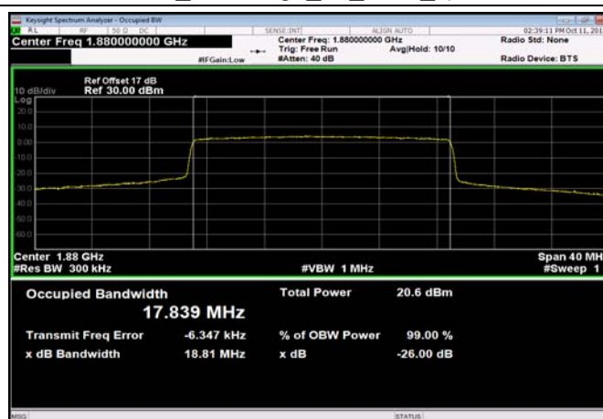
FDD02 MidRange 20 1880 QPSK
