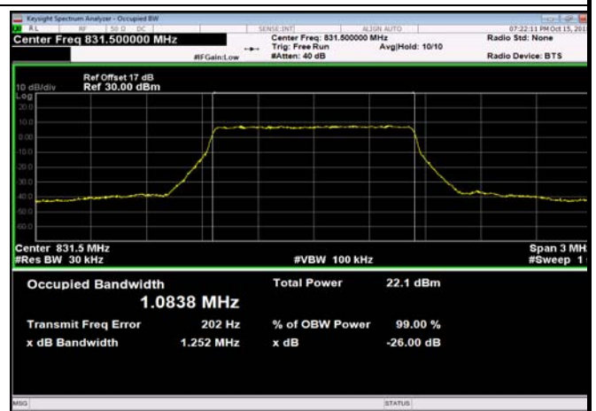
FDD26_MidRange_1.4MHz_831.5MHz_Q16
