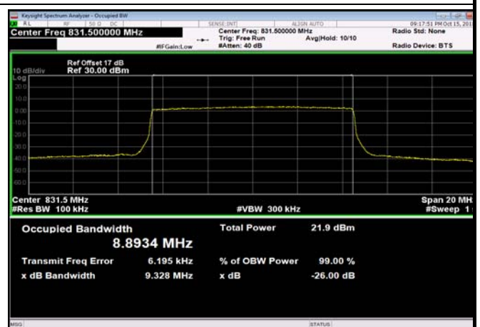
FDD26_MidRange_15_831.5_Q16
