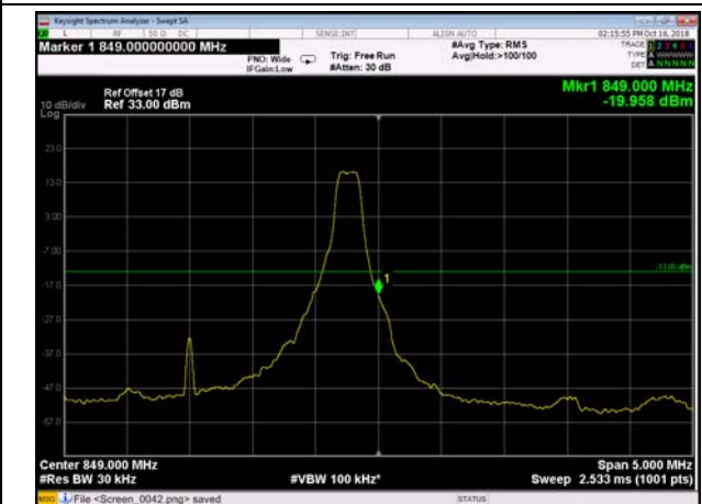
HighRange_FDD26_3MHz_847.5_OneRB _high_Q16
