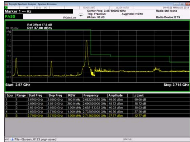
HighRange_TDD41_20MHz_2680_fullRB _HighQPSK
