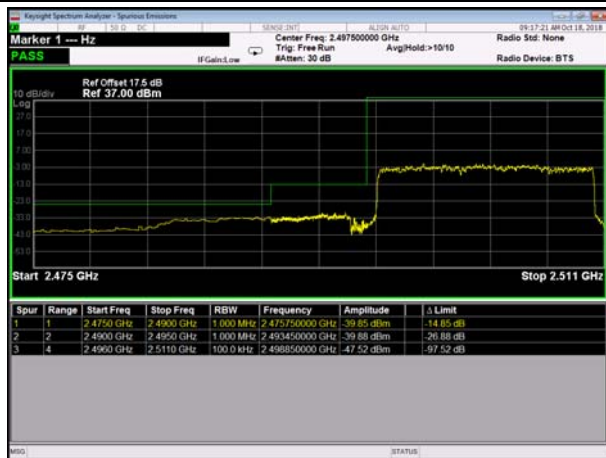
LowRange_TDD41_20MHz_2506_OneRB _low_QPSK
