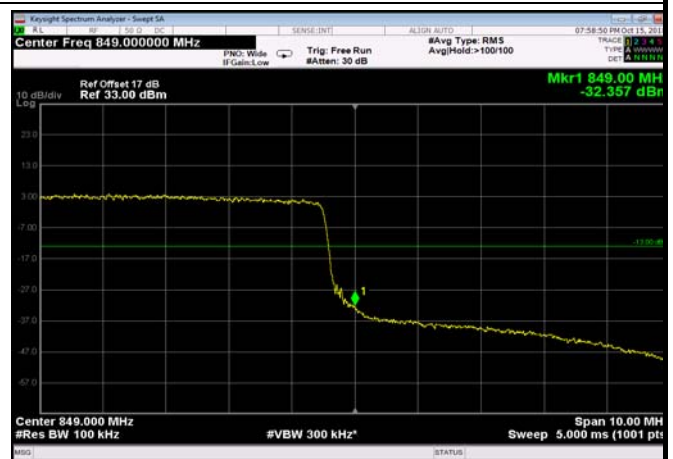
HighRange_FDD26_15MHz_841.5_OneRB _high_Q16
