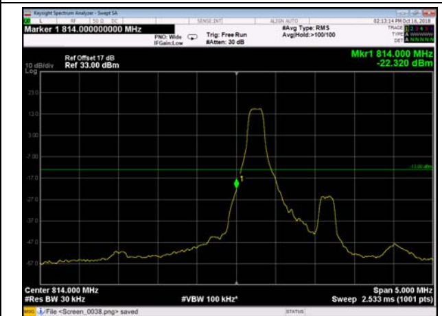
LowRange_FDD26_1.4MHz_814.7_OneRB _low_Q16
