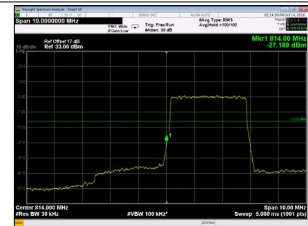
LowRange_FDD26_3MHz_815.5_fullRB _Low_QPSK
