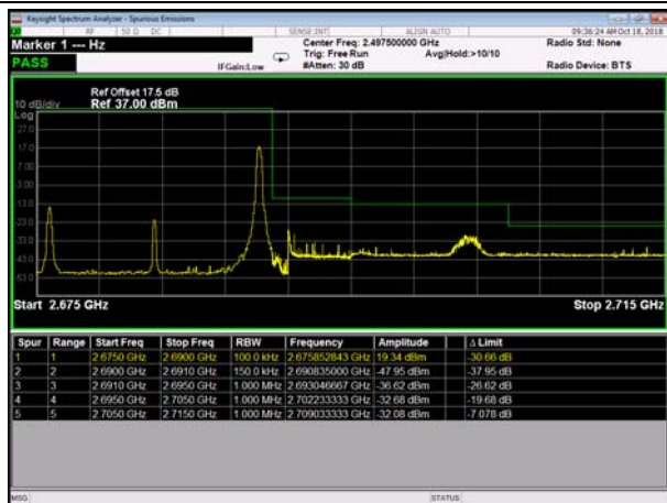
HighRange_TDD41_15MHz_2682.5_fullRB _HighQPSK
