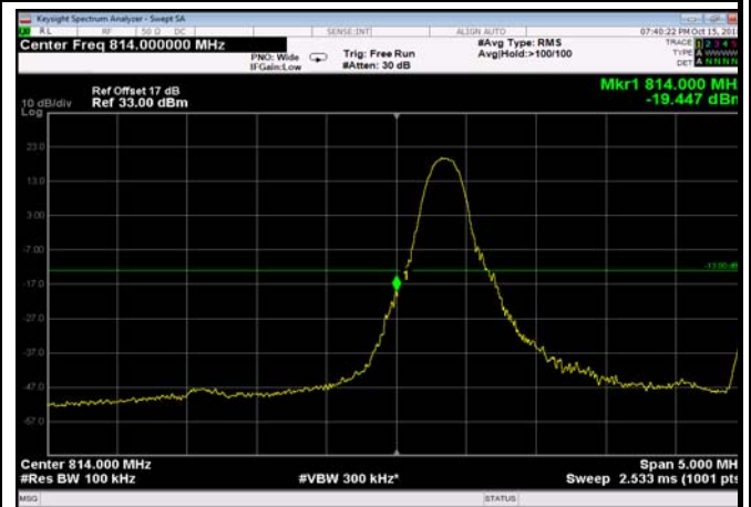
LowRange_FDD26_5MHz_816.5_fullRB _Low_Q16
