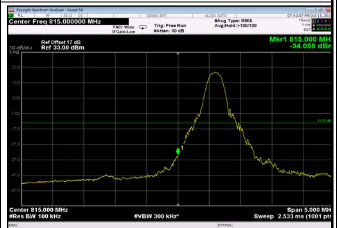
LowRange_FDD26_10MHz_820_OneRB _low_Q16
