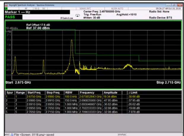
HighRange_TDD41_15MHz_2682.5_fullRB _HighQ16
