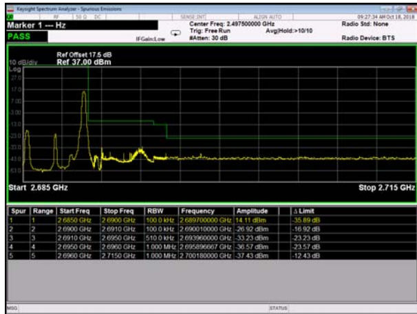
HighRange_TDD41_5MHz_2687.5_fullRB _HighQPSK
