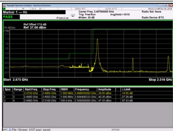
LowRange_TDD41_20MHz_2506_fullRB _LowQPSK
