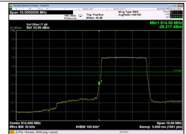
LowRange_FDD26_3MHz_815.5_fullRB _Low_Q16
