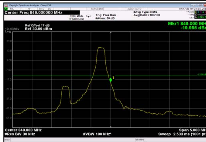
HighRange_FDD26_1.4MHz_848.3_fullRB _High_QPSK
