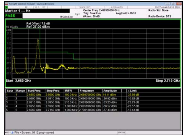
HighRange_TDD41_5MHz_2687.5_fullRB _HighQ16
