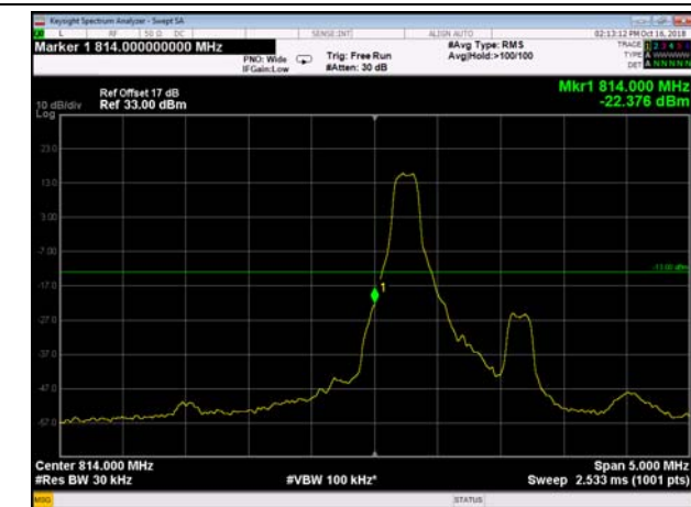
LowRange_FDD26_1.4MHz_814.7_OneRB _low_QPSK
