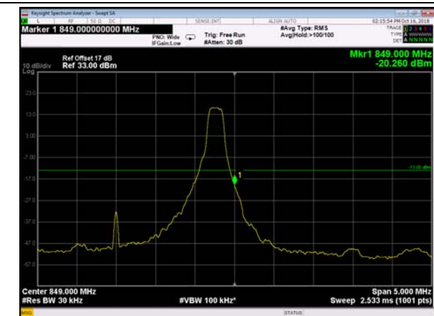
HighRange_FDD26_3MHz_847.5_OneRB _high_QPSK
