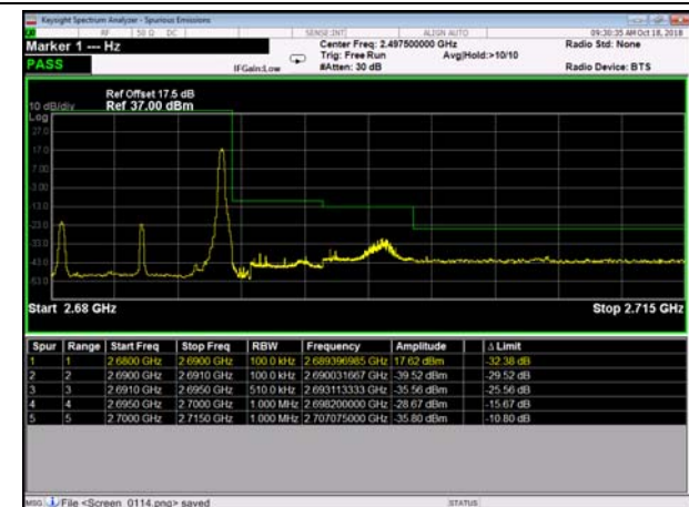
HighRange_TDD41_10MHz_2685_OneRB _high_Q16
