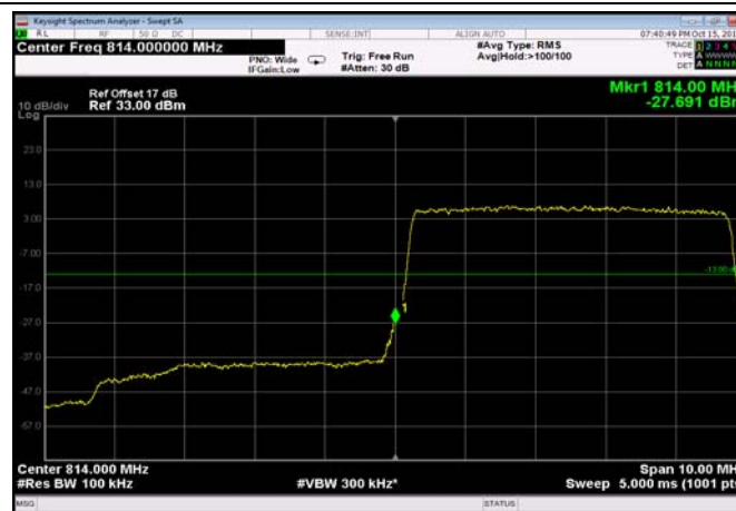
LowRange_FDD26_10MHz_820_OneRB _low_QPSK
