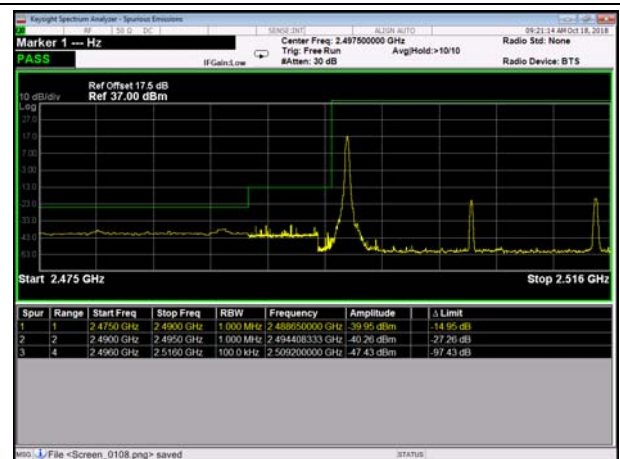
LowRange_TDD41_20MHz_2506_fullRB _LowQ16
