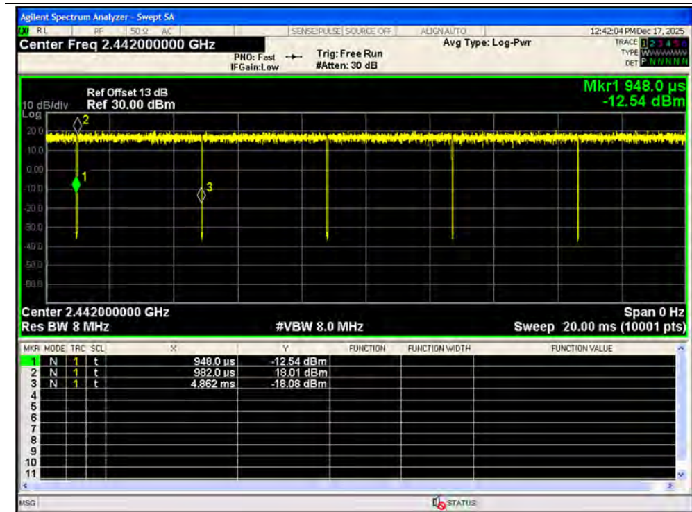
Duty Cycle NVNT ax20 2442MHz Ant1
