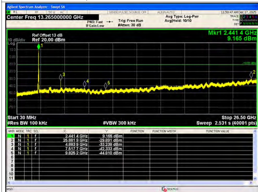
Tx. Spurious NVNT b 2442MHz Ant1 Emission
