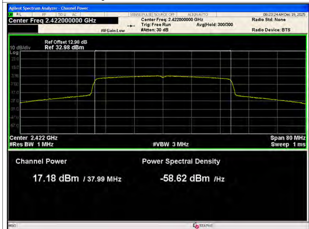
Average Power NVNT ax40 2422MHz Ant1
