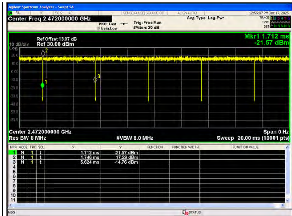
Duty Cycle NVNT ax20 2472MHz Ant1
