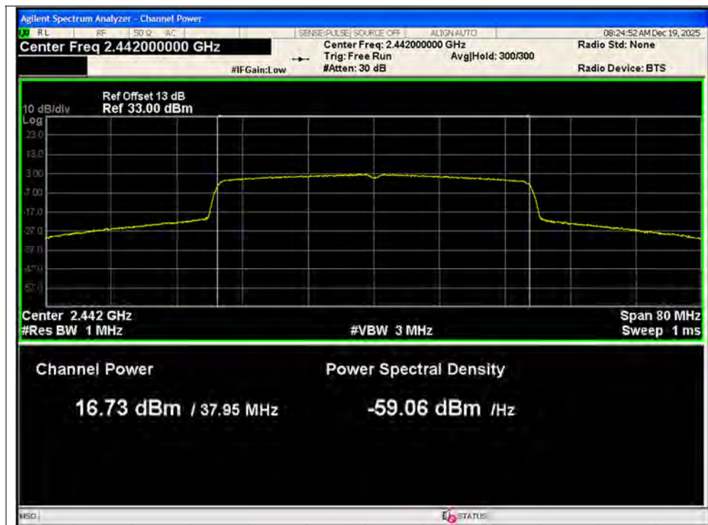
Average Power NVNT ax40 2442MHz Ant1
