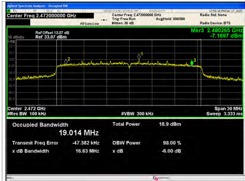
-6dB Bandwidth NVNT ax20 2472MHz Ant1
