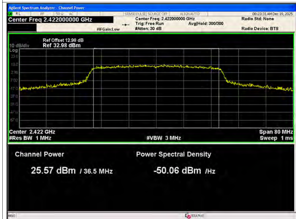
Peak Power NVNT ax40 2422MHz Ant1
