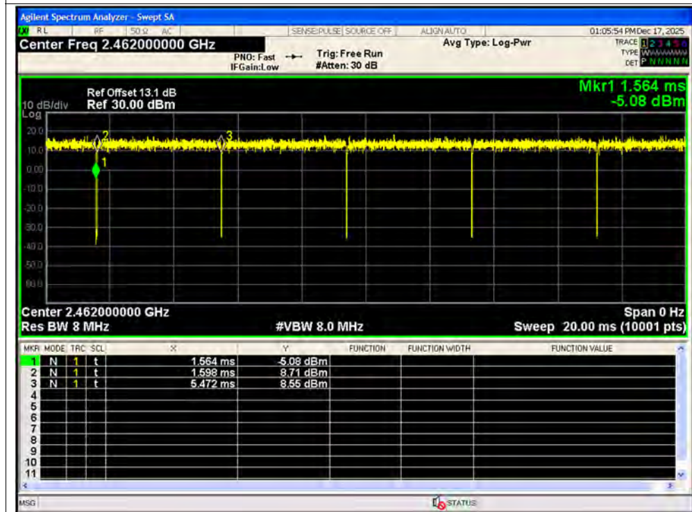
Duty Cycle NVNT ax40 2462MHz Ant1
