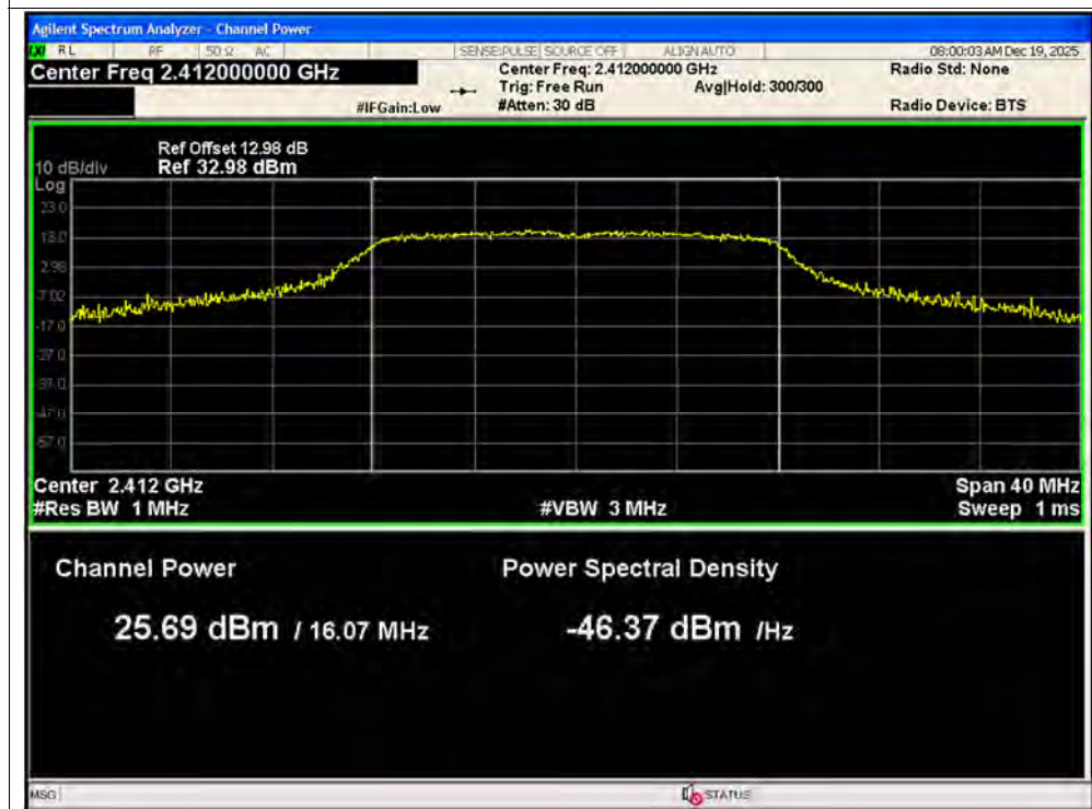
Peak Power NVNT g 2412MHz Ant1
