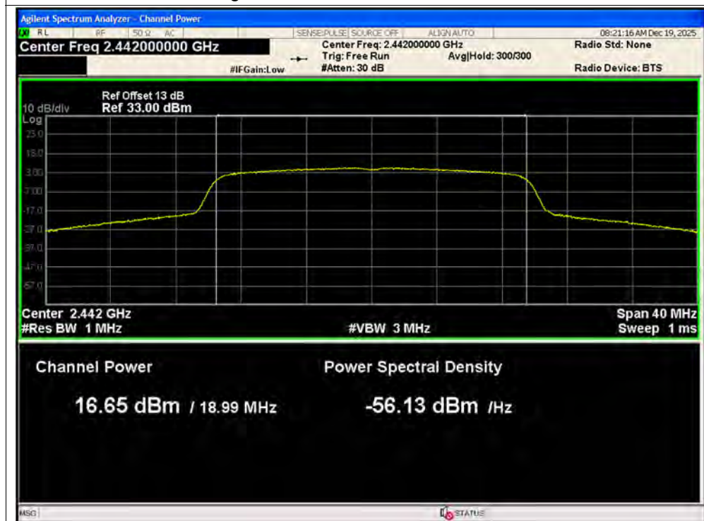
Average Power NVNT ax20 2442MHz Ant1
