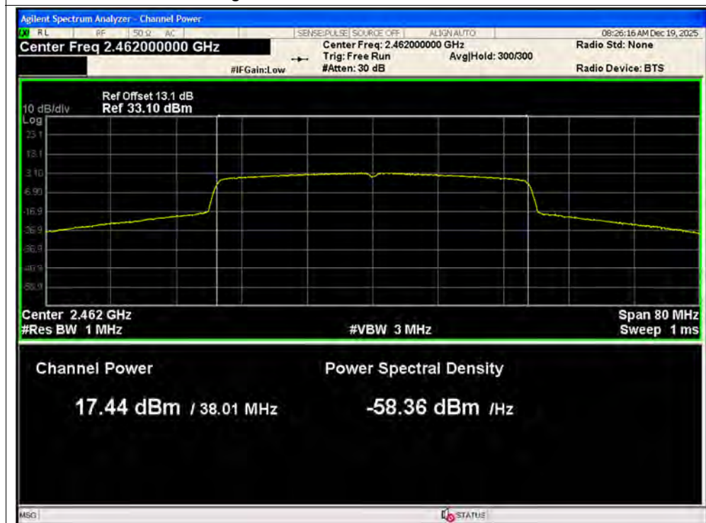
Average Power NVNT ax40 2462MHz Ant1
