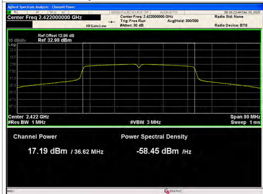
Average Power NVNT n40 2422MHz Ant1
