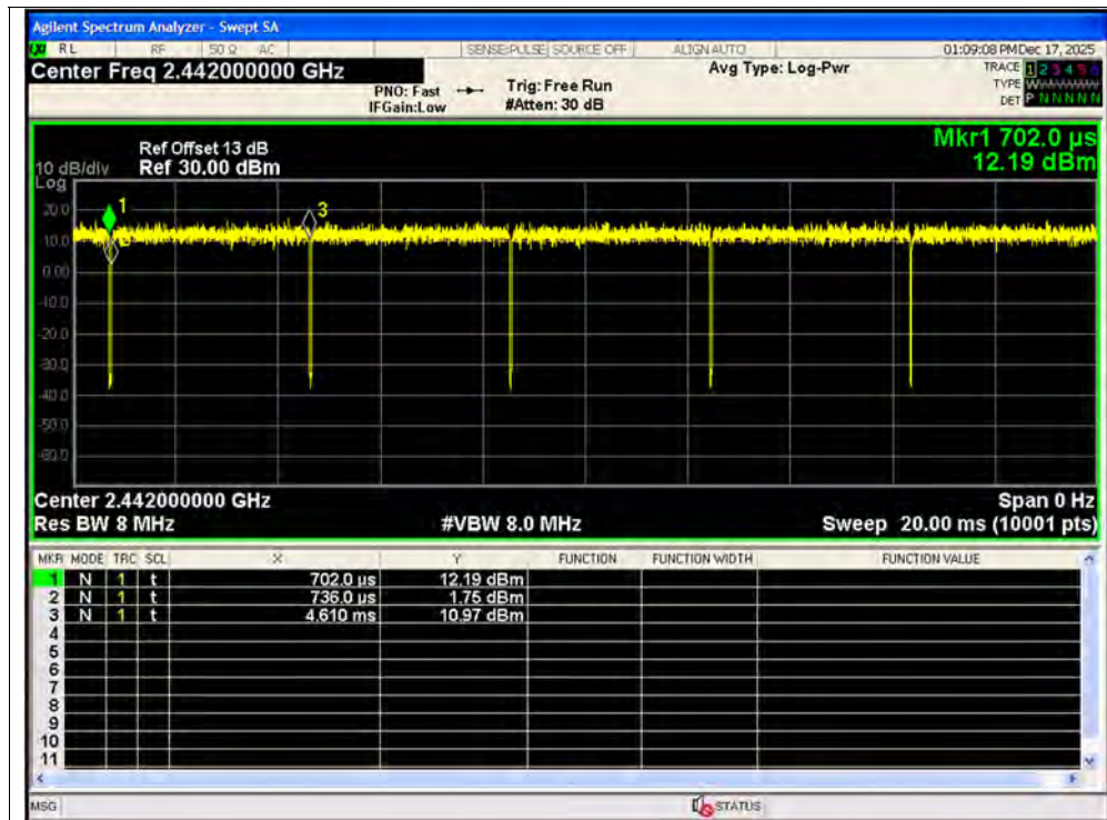
Duty Cycle NVNT ax40 2442MHz Ant1
