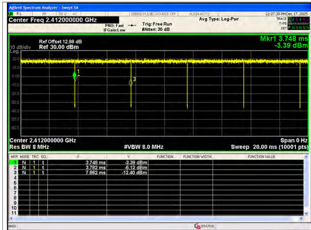
Duty Cycle NVNT ax20 2412MHz Ant1
