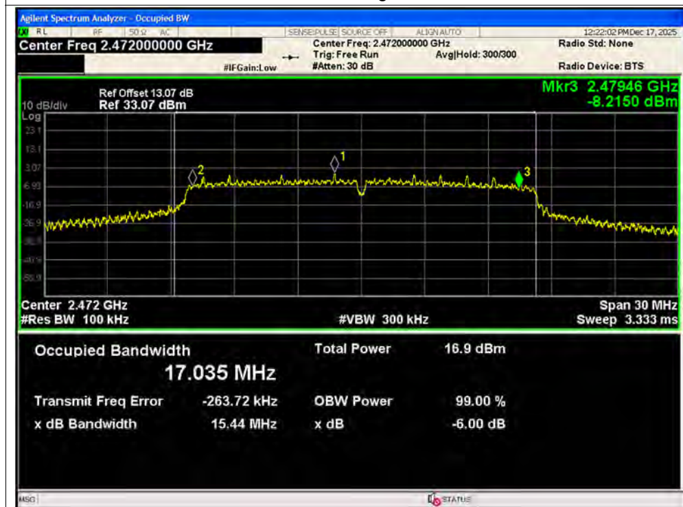
-6dB Bandwidth NVNT g 2472MHz Ant1
