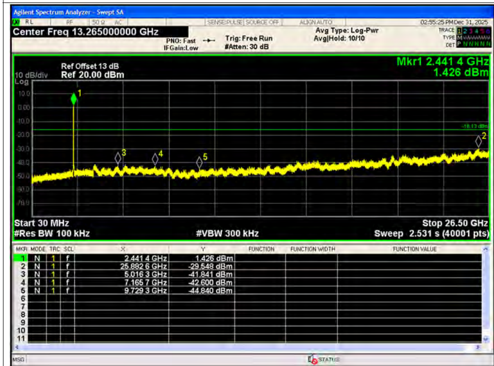
Tx. Spurious NVNT ax20 2442MHz Ant1 Emission
