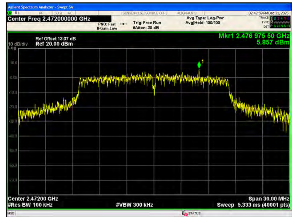
Tx. Spurious NVNT g 2472MHz Ant1 Ref
