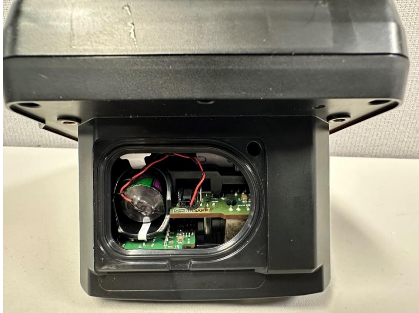
Figure 5 Assembled unit viewed from the rear side (cover removed)
