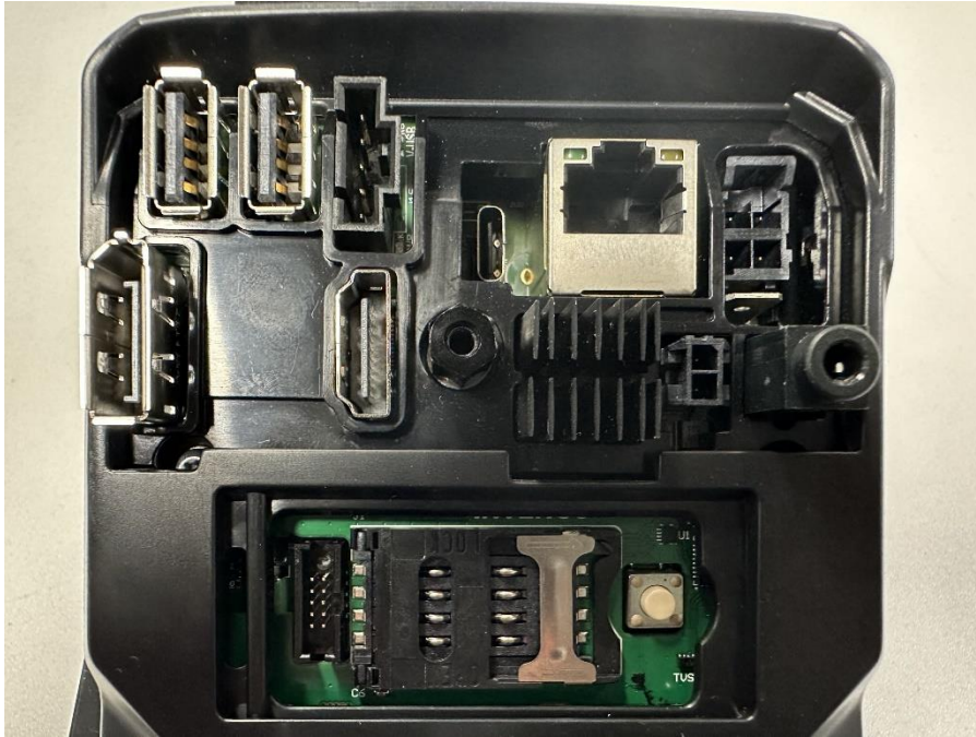
Figure 7 Assembled unit close-up viewed from the back side
