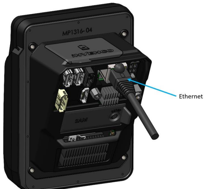
Ethernet Connection
