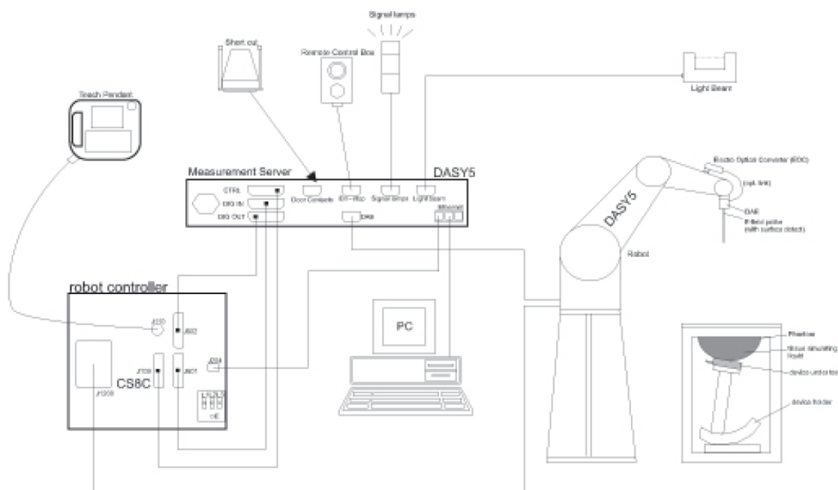
F-1. SAR System Configuration
