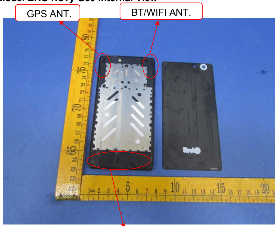
EUT –Model EKO Novy G50 Internal View
