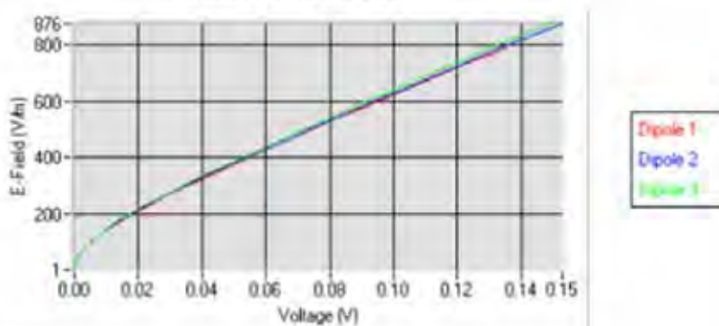
Calibration curves
