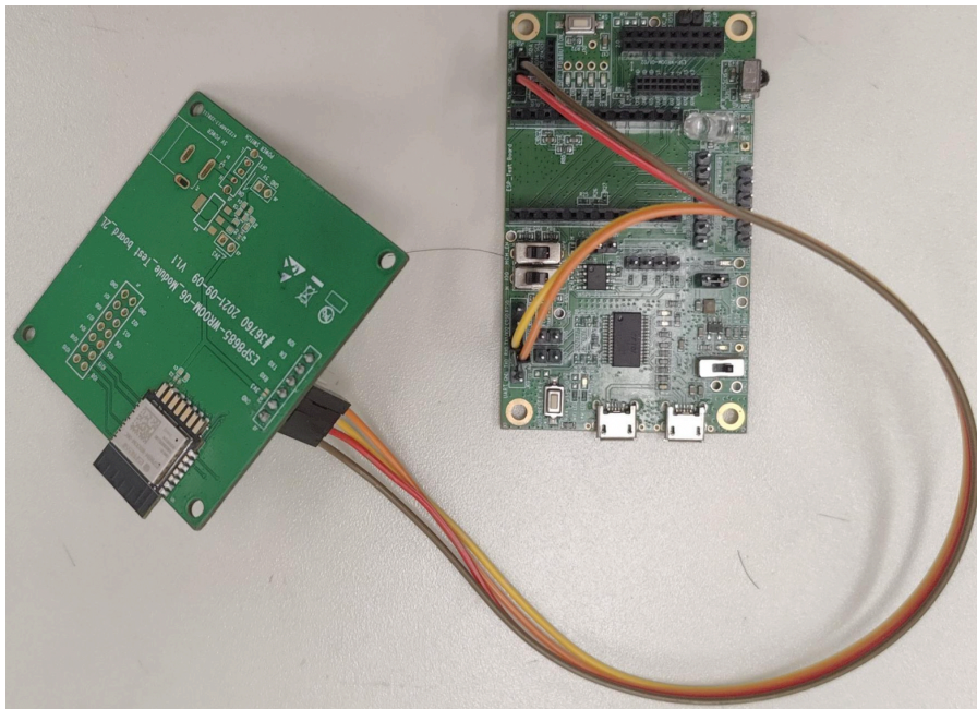
Figure 2: Hardware Connection
