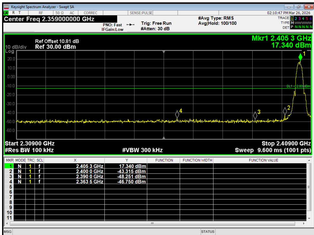
Band Edge Thread 2405MHz Emission
