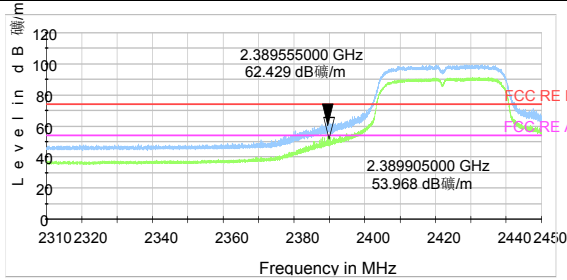
802.11n HT40 -Channel 3 Peak+ Average
