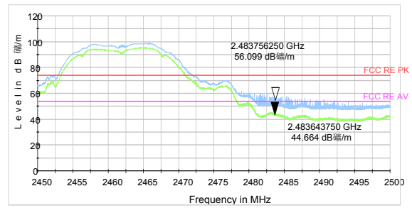
802.11b-Channel 11 Peak+ Average
