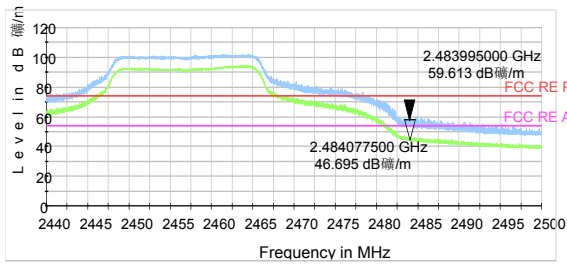
802.11n HT20 -Channel 10 Peak+ Average
