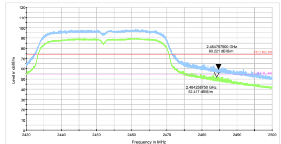
802.11n HT40 -Channel 9 Peak+ Average
