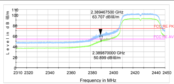
802.11n HT40 -Channel 4 Peak+ Average
