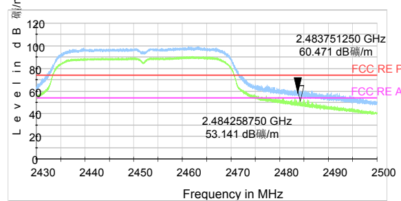
802.11n HT40 -Channel 9 Peak+ Average
