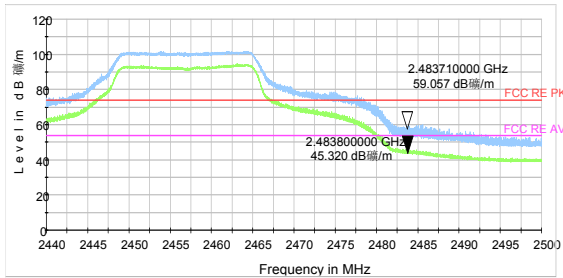
802.11g-Channel 10 Peak+ Average
