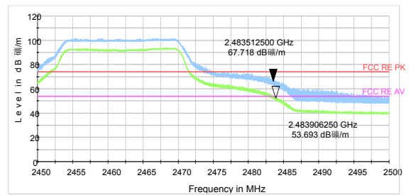
802.11g-Channel 11 Peak+ Average
