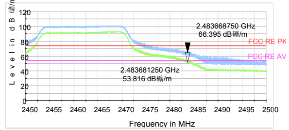
802.11n HT20 -Channel 11 Peak+ Average
