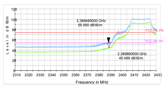
802.11g-Channel 2 Peak+ Average
