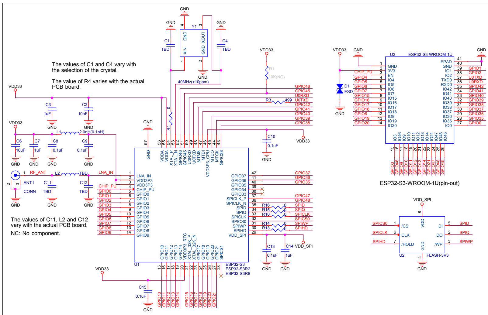
Figure 6: ESP32-S3-WROOM-1U Schematics
