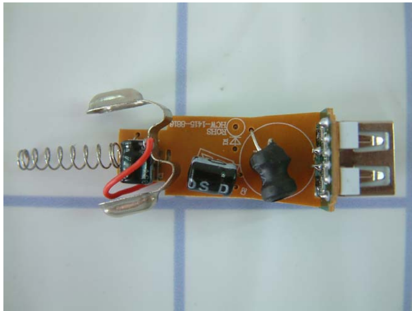
Charger PCB side 1 view
