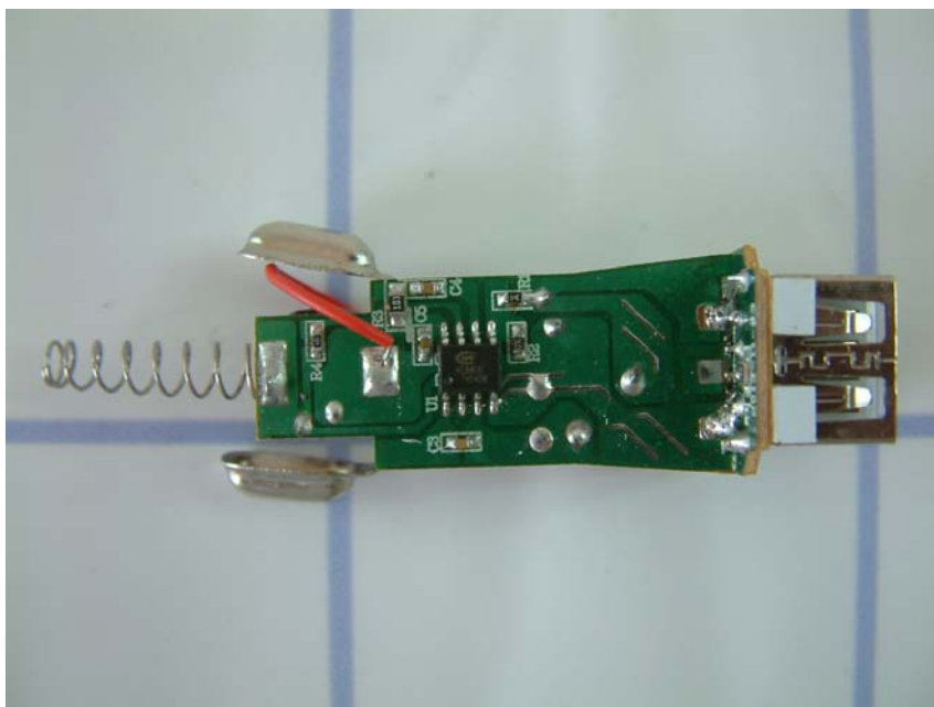
Charger PCB side 2 view
