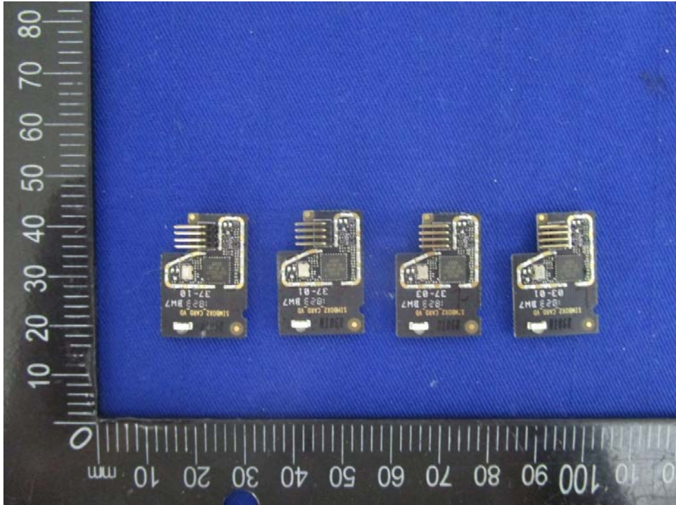
EUT – SIM Card Slot Bottom View
