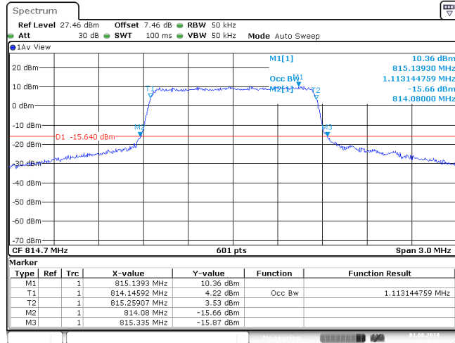
Band26_1.4MHz_QPSK_26697_6RB#0
