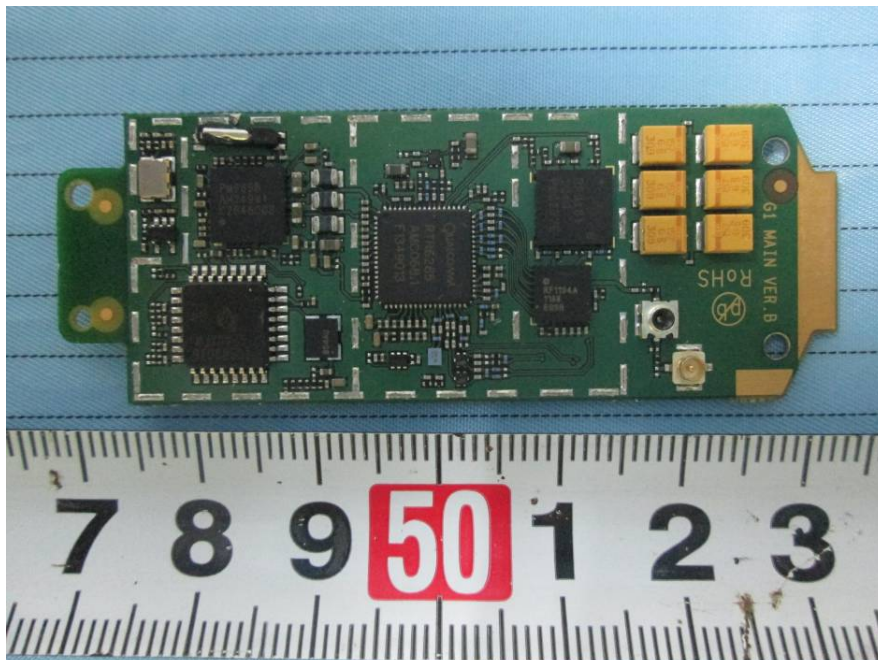
EUT – Main Board Bottom 2 Shielding off View
