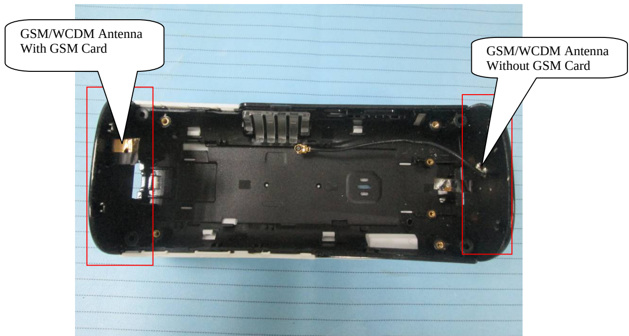
EUT – Antenna View
