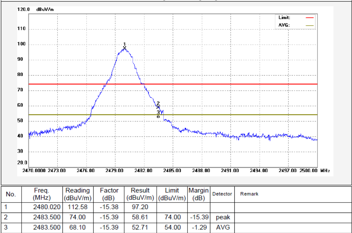
Pi/4 DQPSK Transmitting Band edge-right side Vertical
