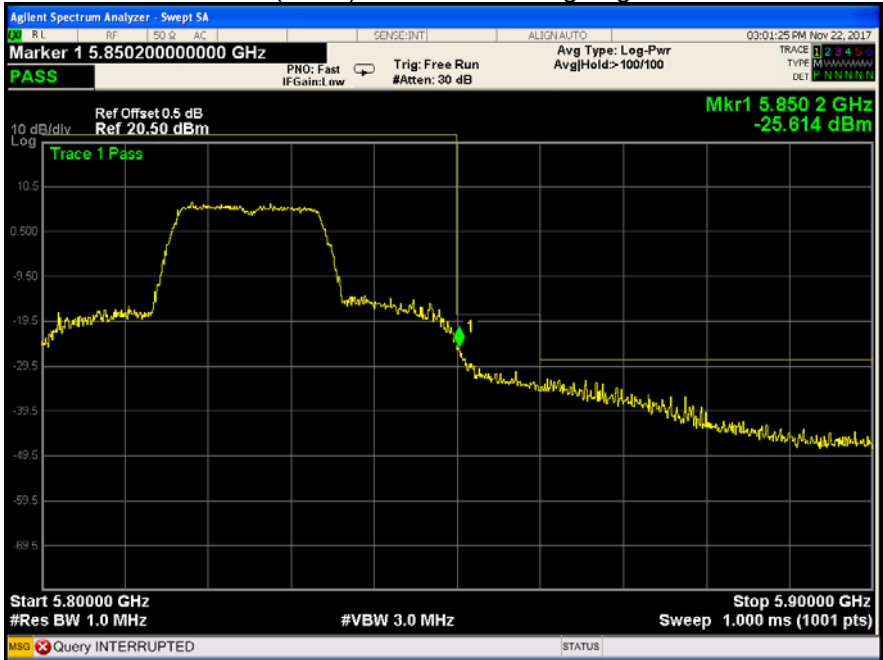
802.11n(HT20) band IV Band edge-right side
