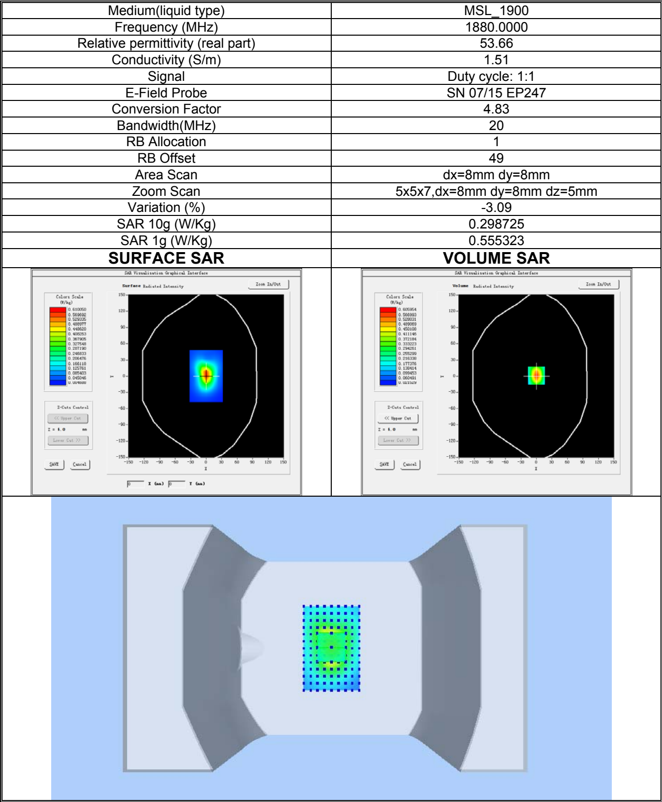
Plot 16:LTE BAND2, Middle channel (Hotspot, Bottom Edge) Product Description:4G Wireless Data Terminal Test Date: 2019-09-11
