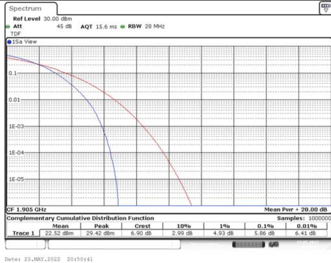
Band25-20MHz-16QAM-26590-100RB#0
