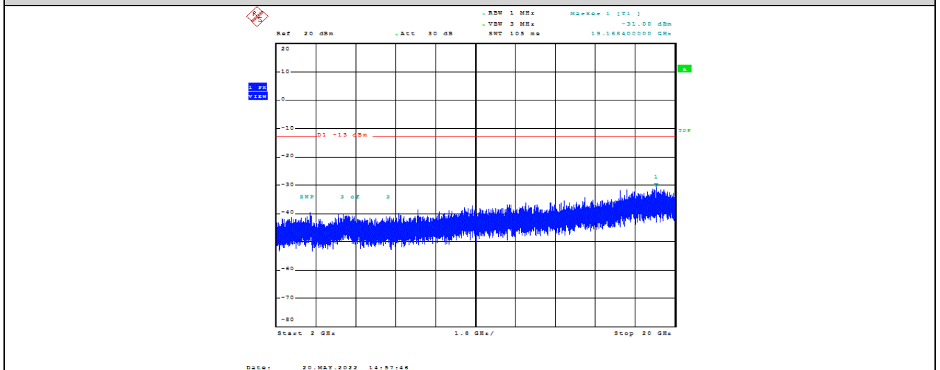
Band25-1.4MHz-QPSK-26047-1RB#0-Range3:2000~20000MHz
