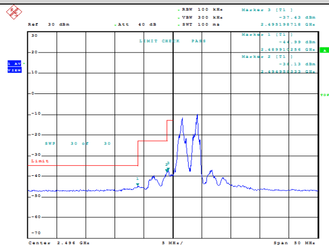
Band41-5MHz-QPSK-39675-1RB#24
