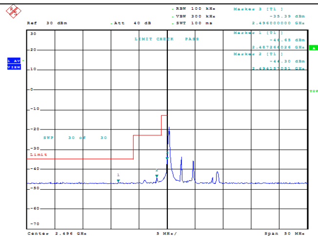
Band41-5MHz-QPSK-39675-1RB#0
