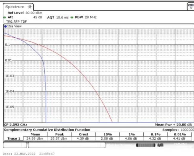
Band41-5MHz-QPSK-40620-1RB#0
