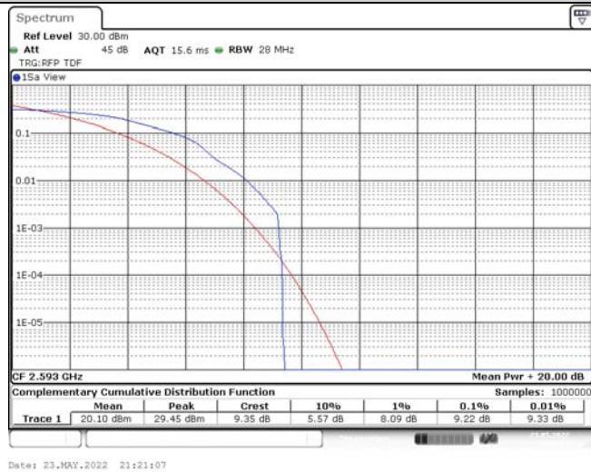
Band41-15MHz-16QAM-40620-1RB#0
